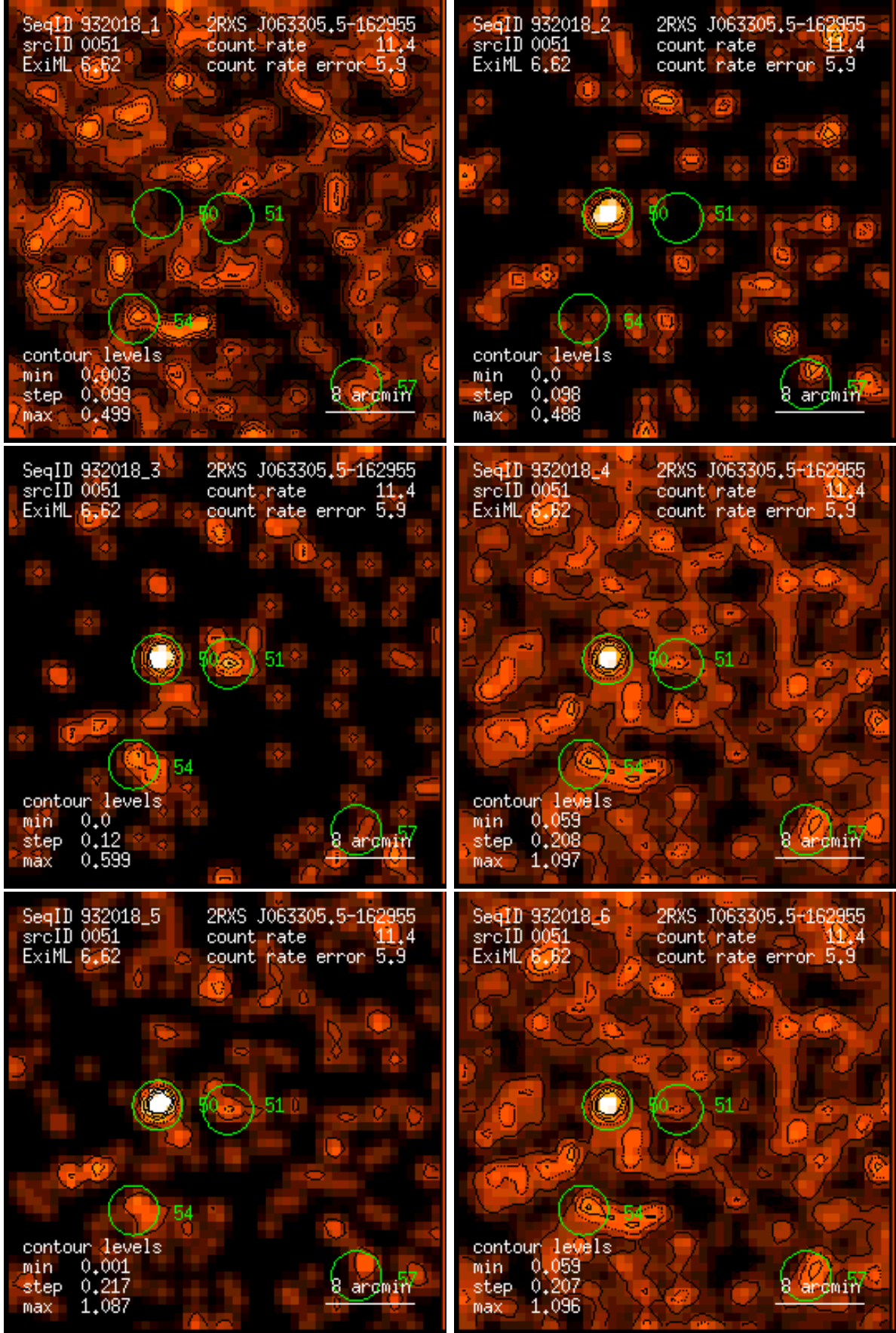
Figure 51: RASS 932018: detection 0051: band rate images, Gaussian filter: (1) PSPC channels 11 – 41, (2) 52 – 90, (3) 91 – 201, (4) 11 – 235, (5) 52 – 201, (6) 11 – 201. Broad band rates in counts/ks. Band rate contour levels in counts/ks/arcmin 2 .
