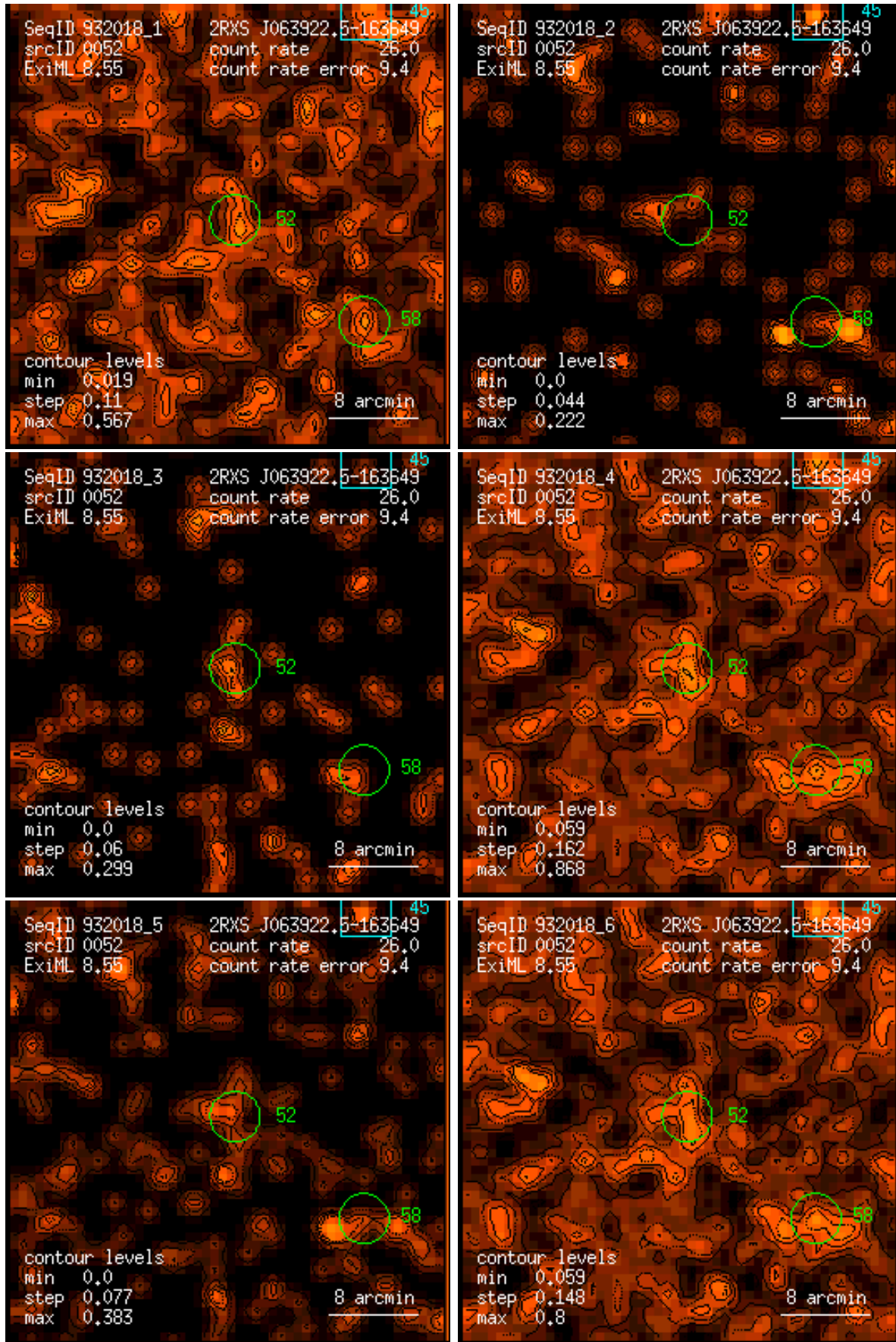
Figure 52: RASS 932018: detection 0052: band rate images, Gaussian filter: (1) PSPC channels 11 – 41, (2) 52 – 90, (3) 91 – 201, (4) 11 – 235, (5) 52 – 201, (6) 11 – 201. Broad band rates in counts/ks. Band rate contour levels in counts/ks/arcmin 2 .
