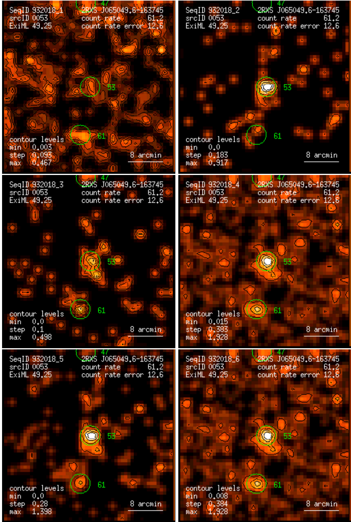
Figure 53: RASS 932018: detection 0053: band rate images, Gaussian filter: (1) PSPC channels 11 – 41, (2) 52 – 90, (3) 91 – 201, (4) 11 – 235, (5) 52 – 201, (6) 11 – 201. Broad band rates in counts/ks. Band rate contour levels in counts/ks/arcmin 2 .
