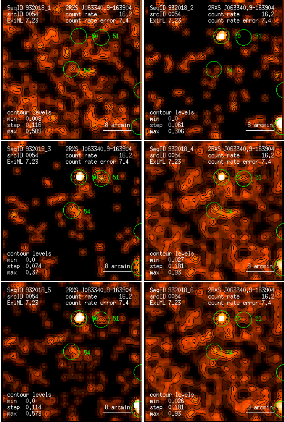
Figure 54: RASS 932018: detection 0054: band rate images, Gaussian filter: (1) PSPC channels 11 – 41, (2) 52 – 90, (3) 91 – 201, (4) 11 – 235, (5) 52 – 201, (6) 11 – 201. Broad band rates in counts/ks. Band rate contour levels in counts/ks/arcmin 2 .
