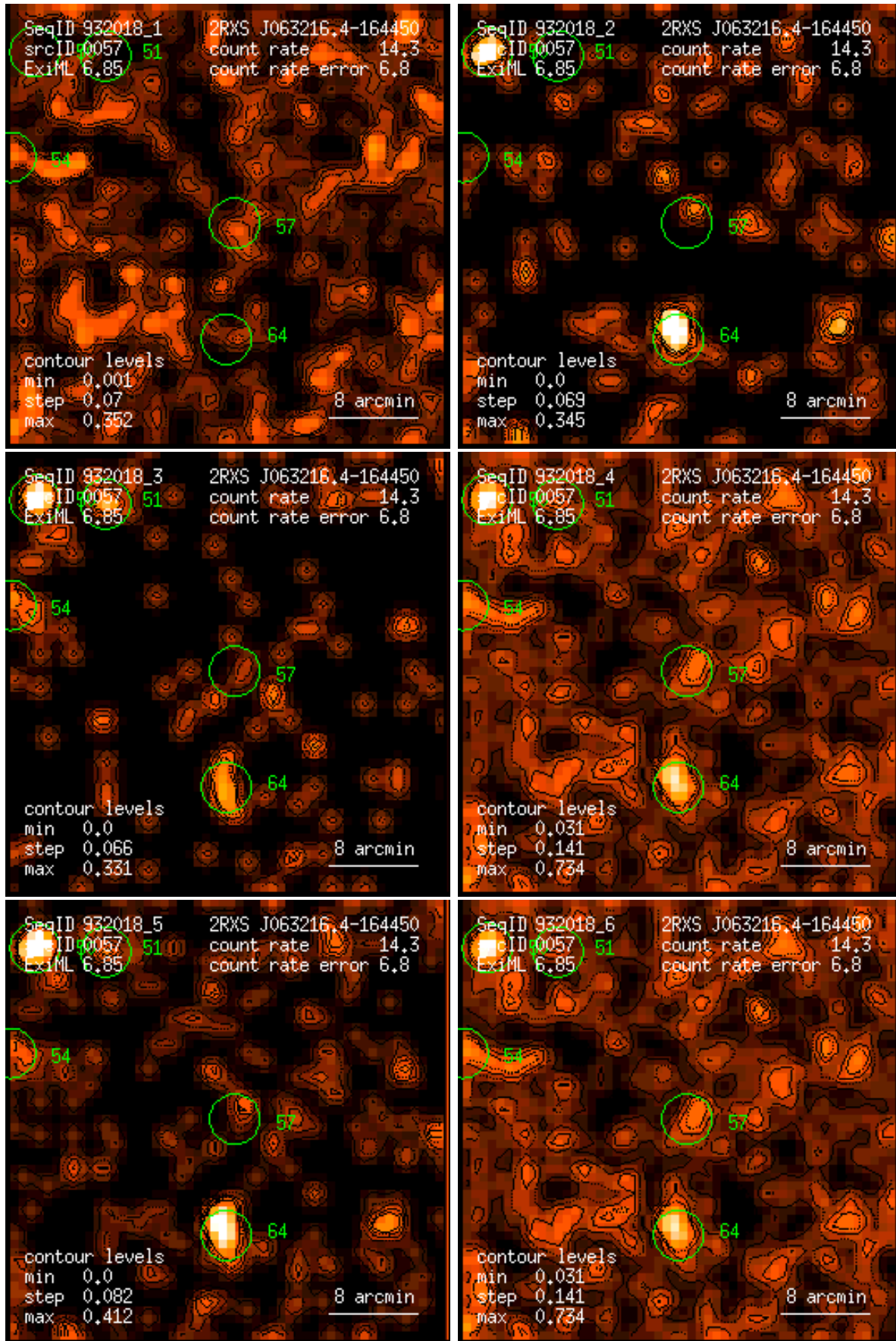
Figure 57: RASS 932018: detection 0057: band rate images, Gaussian filter: (1) PSPC channels 11 – 41, (2) 52 – 90, (3) 91 – 201, (4) 11 – 235, (5) 52 – 201, (6) 11 – 201. Broad band rates in counts/ks. Band rate contour levels in counts/ks/arcmin 2 .
