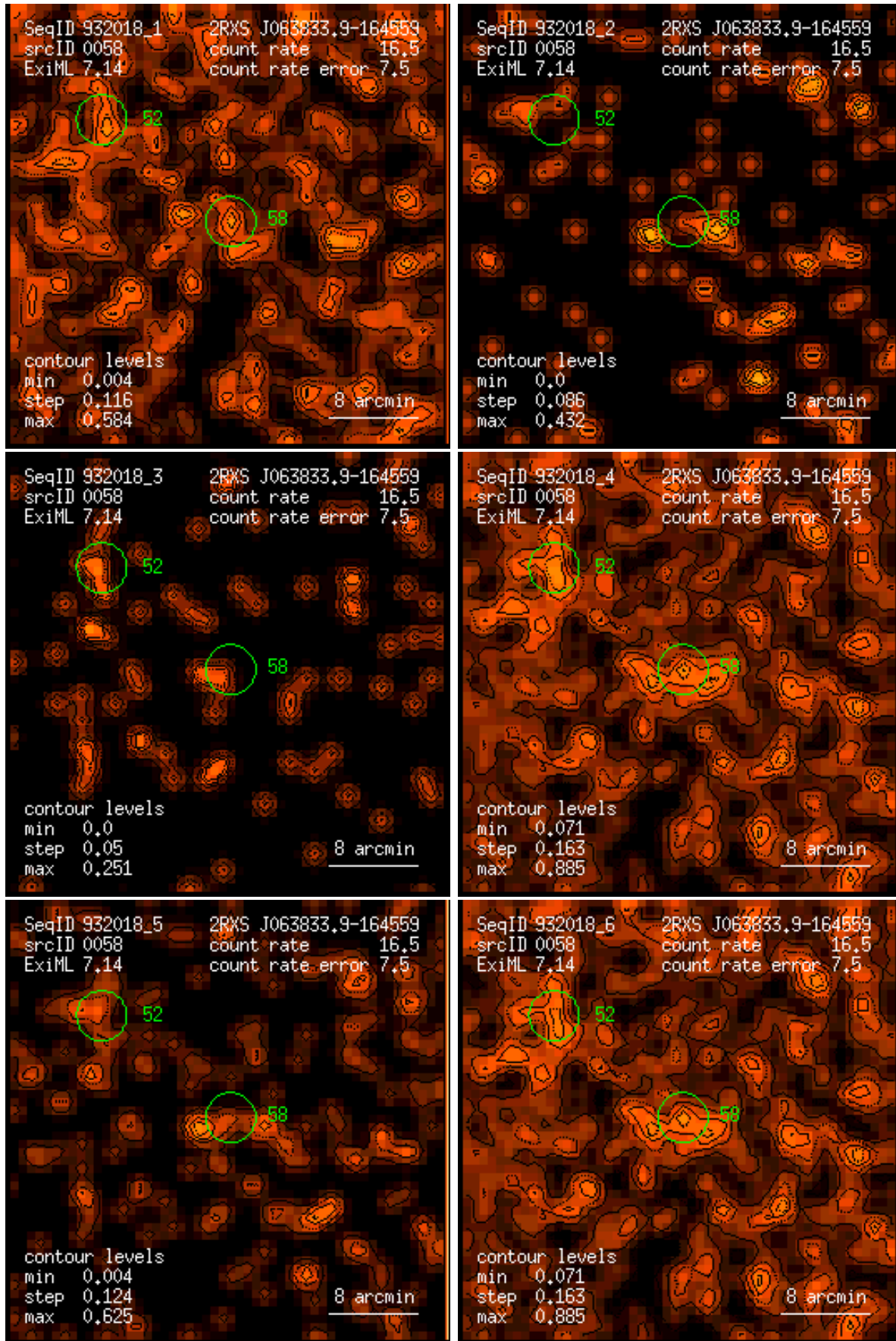
Figure 58: RASS 932018: detection 0058: band rate images, Gaussian filter: (1) PSPC channels 11 – 41, (2) 52 – 90, (3) 91 – 201, (4) 11 – 235, (5) 52 – 201, (6) 11 – 201. Broad band rates in counts/ks. Band rate contour levels in counts/ks/arcmin 2 .
