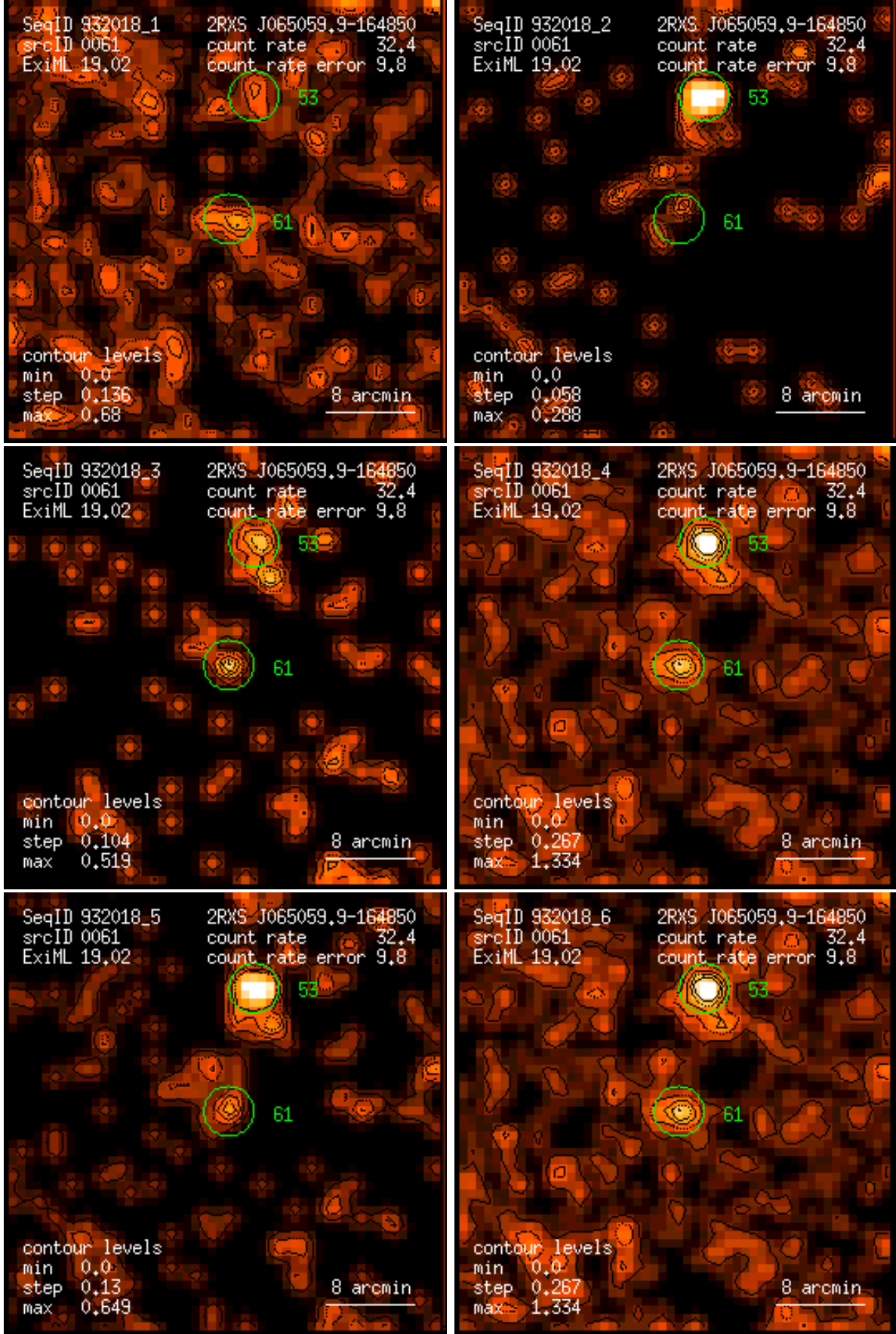
Figure 61: RASS 932018: detection 0061: band rate images, Gaussian filter: (1) PSPC channels 11 – 41, (2) 52 – 90, (3) 91 – 201, (4) 11 – 235, (5) 52 – 201, (6) 11 – 201. Broad band rates in counts/ks. Band rate contour levels in counts/ks/arcmin 2 .
