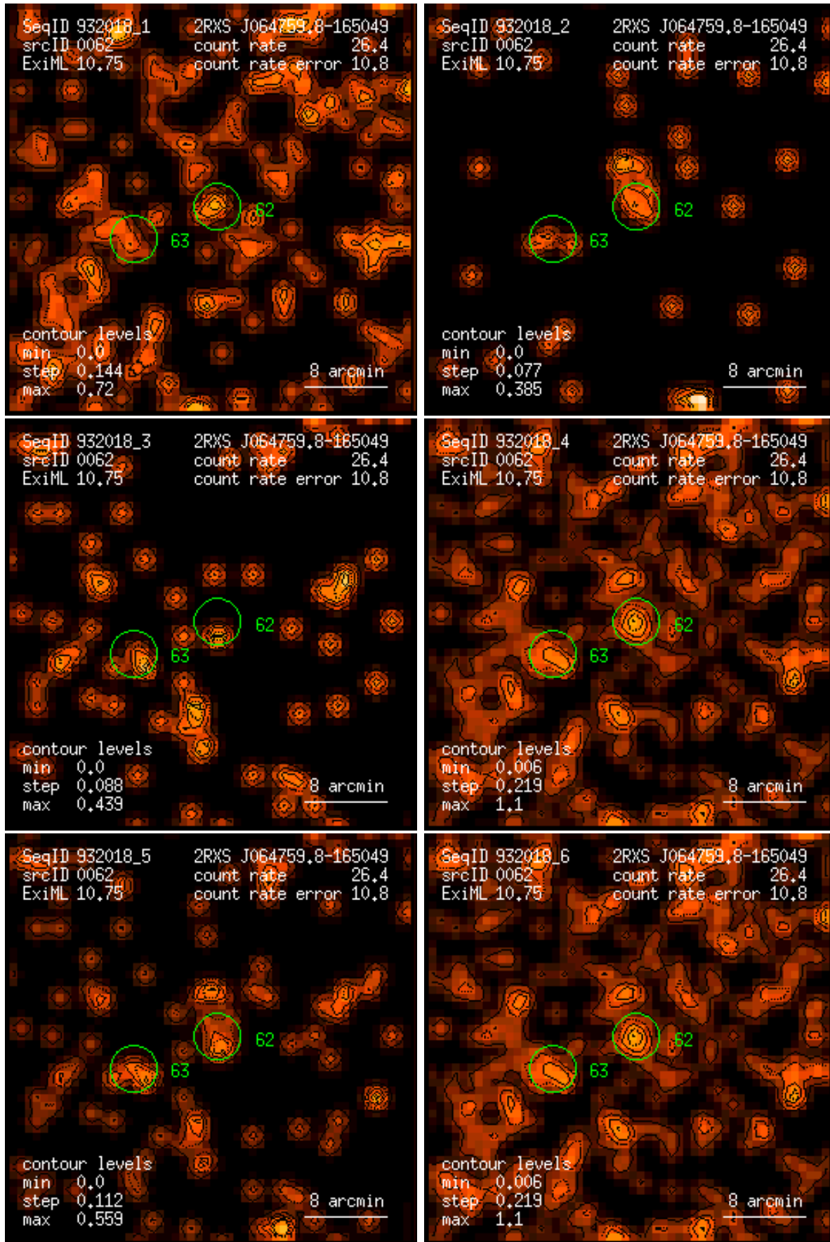
Figure 62: RASS 932018: detection 0062: band rate images, Gaussian filter: (1) PSPC channels 11 – 41, (2) 52 – 90, (3) 91 – 201, (4) 11 – 235, (5) 52 – 201, (6) 11 – 201. Broad band rates in counts/ks. Band rate contour levels in counts/ks/arcmin 2 .
