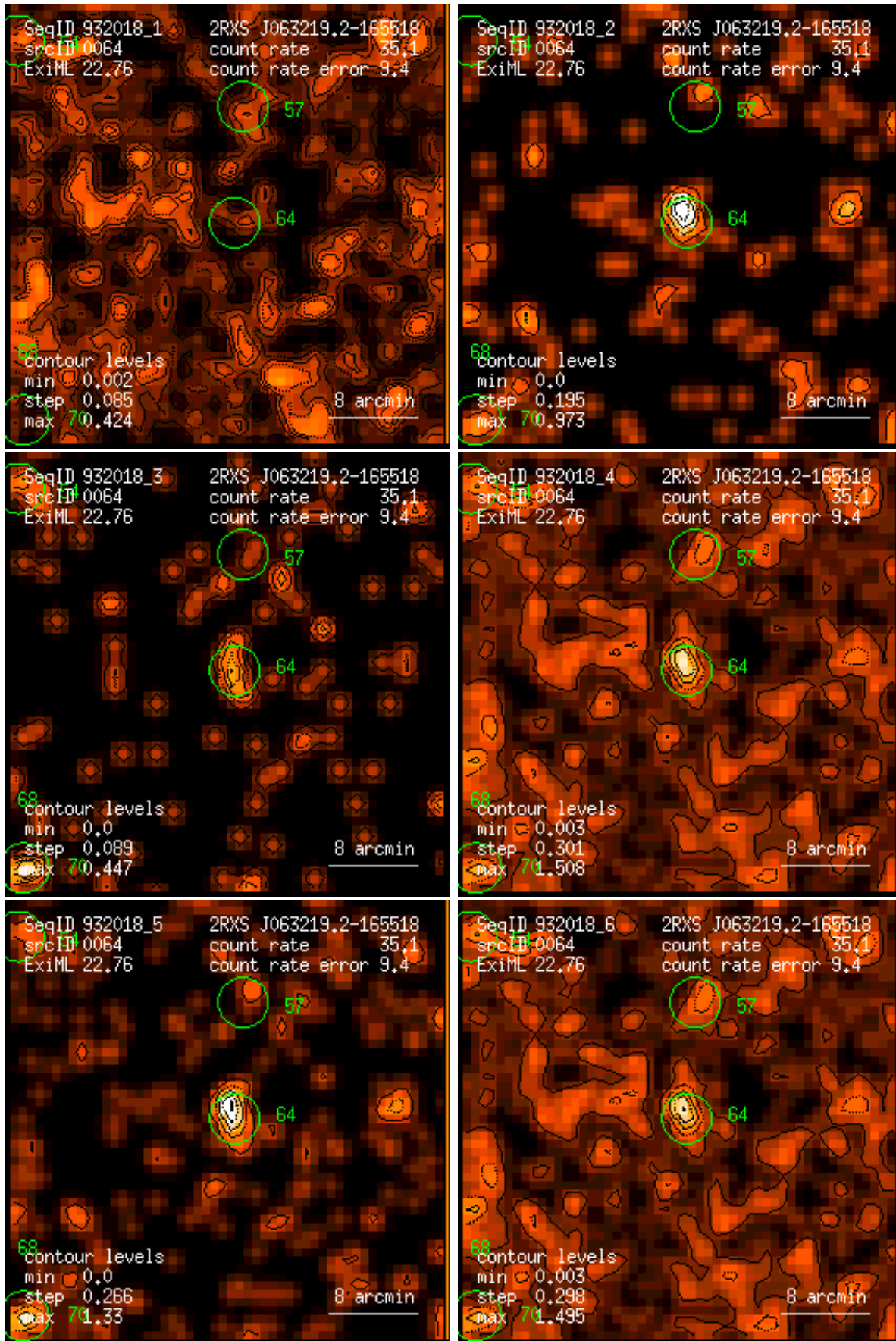
Figure 64: RASS 932018: detection 0064: band rate images, Gaussian filter: (1) PSPC channels 11 – 41, (2) 52 – 90, (3) 91 – 201, (4) 11 – 235, (5) 52 – 201, (6) 11 – 201. Broad band rates in counts/ks. Band rate contour levels in counts/ks/arcmin 2 .
