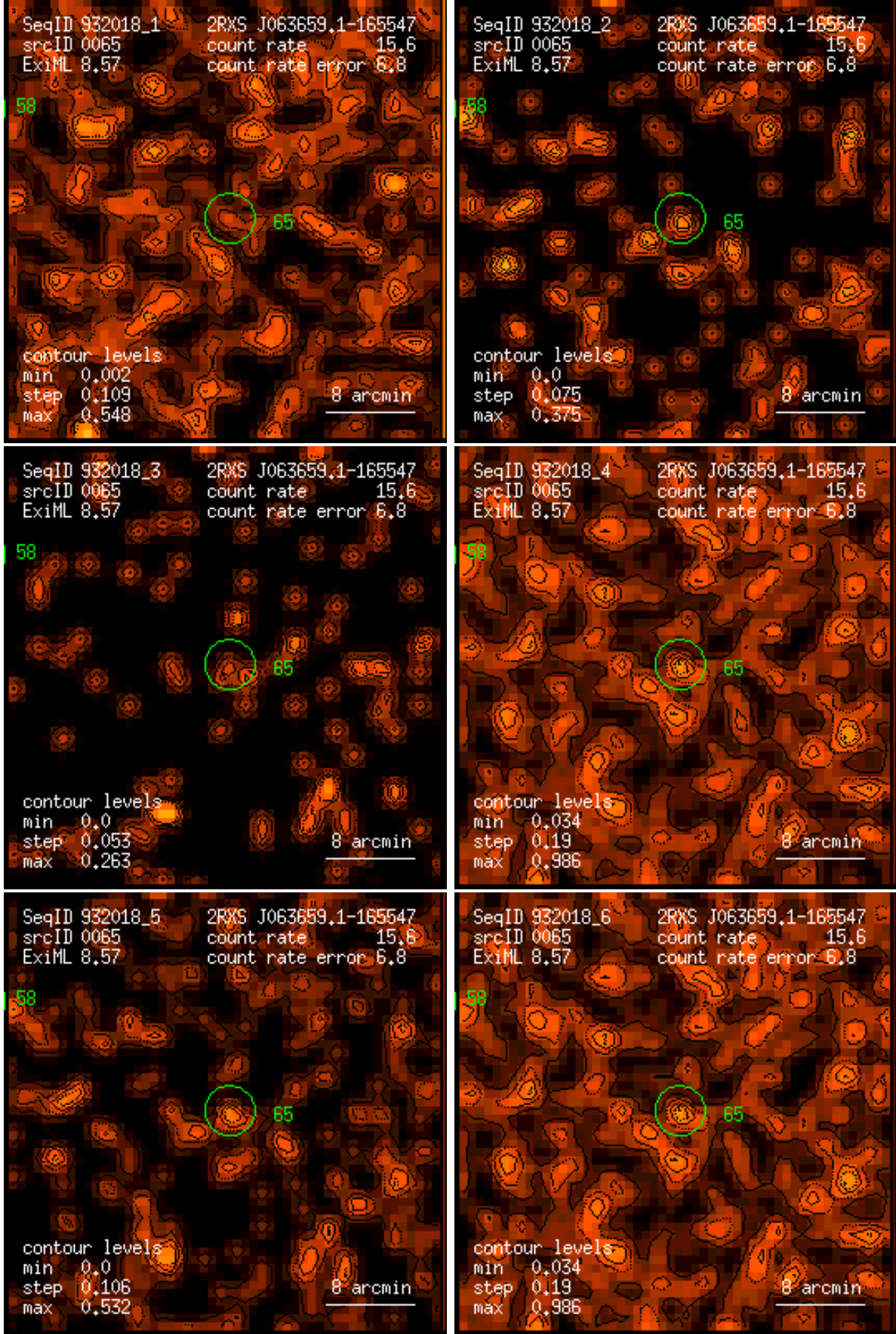
Figure 65: RASS 932018: detection 0065: band rate images, Gaussian filter: (1) PSPC channels 11 – 41, (2) 52 – 90, (3) 91 – 201, (4) 11 – 235, (5) 52 – 201, (6) 11 – 201. Broad band rates in counts/ks. Band rate contour levels in counts/ks/arcmin 2 .
