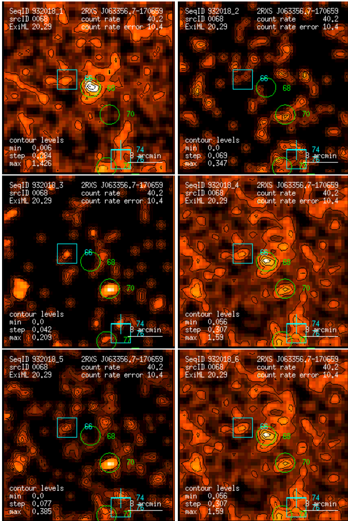
Figure 68: RASS 932018: detection 0068: band rate images, Gaussian filter: (1) PSPC channels 11 – 41, (2) 52 – 90, (3) 91 – 201, (4) 11 – 235, (5) 52 – 201, (6) 11 – 201. Broad band rates in counts/ks. Band rate contour levels in counts/ks/arcmin 2 .
