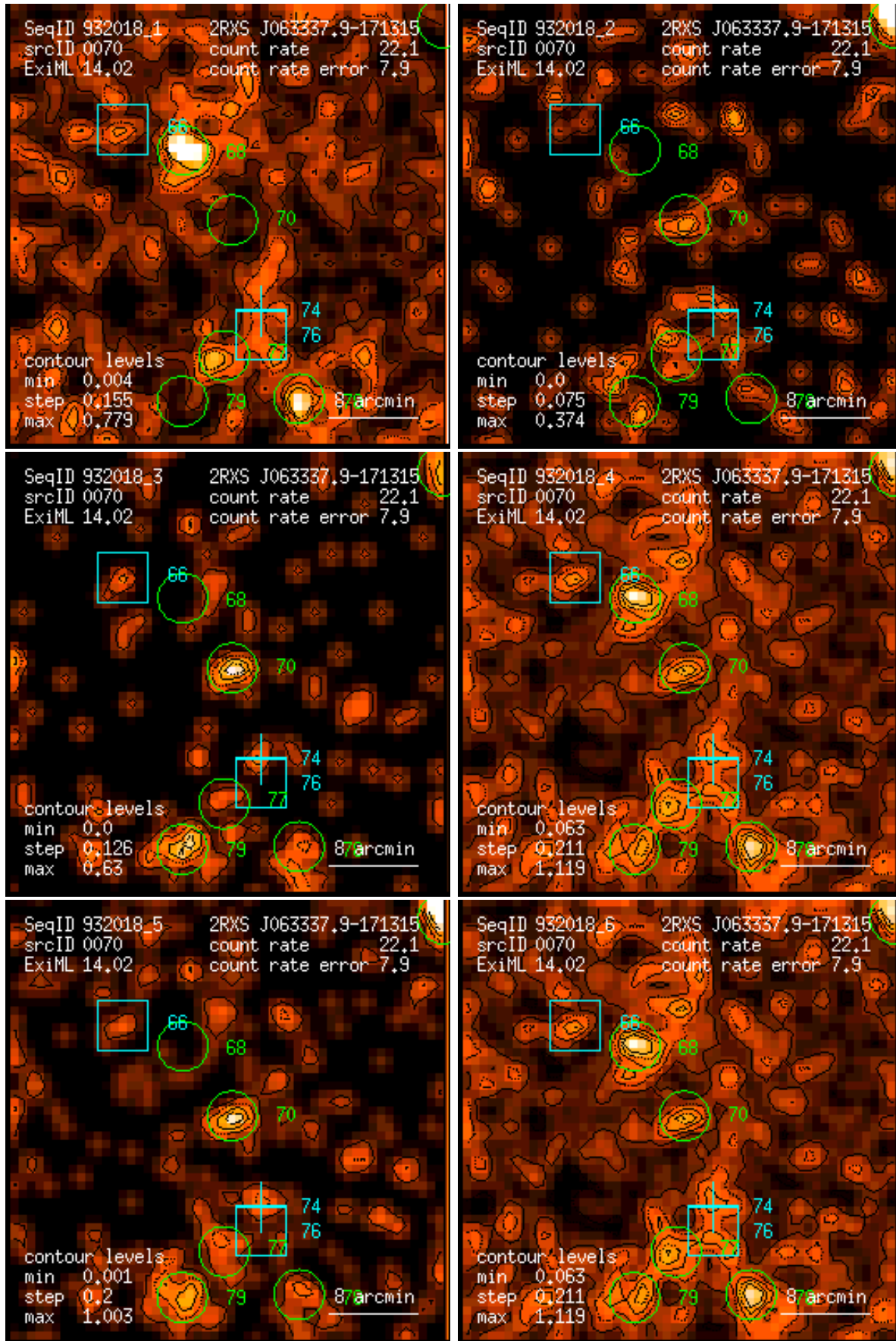
Figure 70: RASS 932018: detection 0070: band rate images, Gaussian filter: (1) PSPC channels 11 – 41, (2) 52 – 90, (3) 91 – 201, (4) 11 – 235, (5) 52 – 201, (6) 11 – 201. Broad band rates in counts/ks. Band rate contour levels in counts/ks/arcmin 2 .
