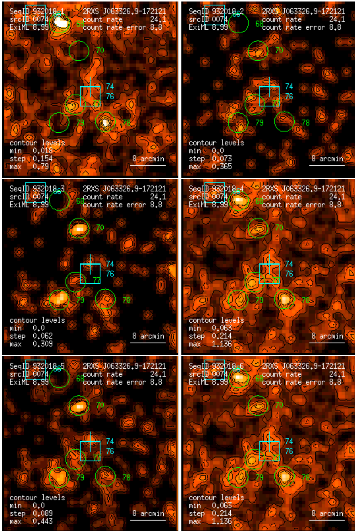
Figure 74: RASS 932018: detection 0074: band rate images, Gaussian filter: (1) PSPC channels 11 – 41, (2) 52 – 90, (3) 91 – 201, (4) 11 – 235, (5) 52 – 201, (6) 11 – 201. Broad band rates in counts/ks. Band rate contour levels in counts/ks/arcmin 2 .
