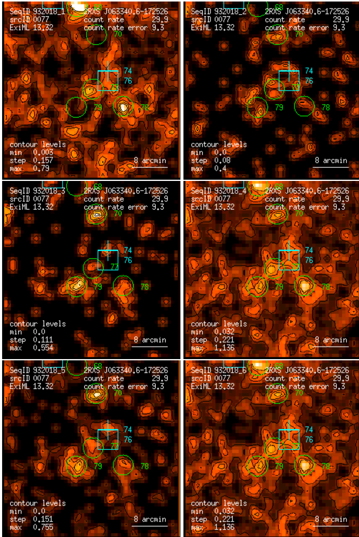
Figure 77: RASS 932018: detection 0077: band rate images, Gaussian filter: (1) PSPC channels 11 – 41, (2) 52 – 90, (3) 91 – 201, (4) 11 – 235, (5) 52 – 201, (6) 11 – 201. Broad band rates in counts/ks. Band rate contour levels in counts/ks/arcmin 2 .
