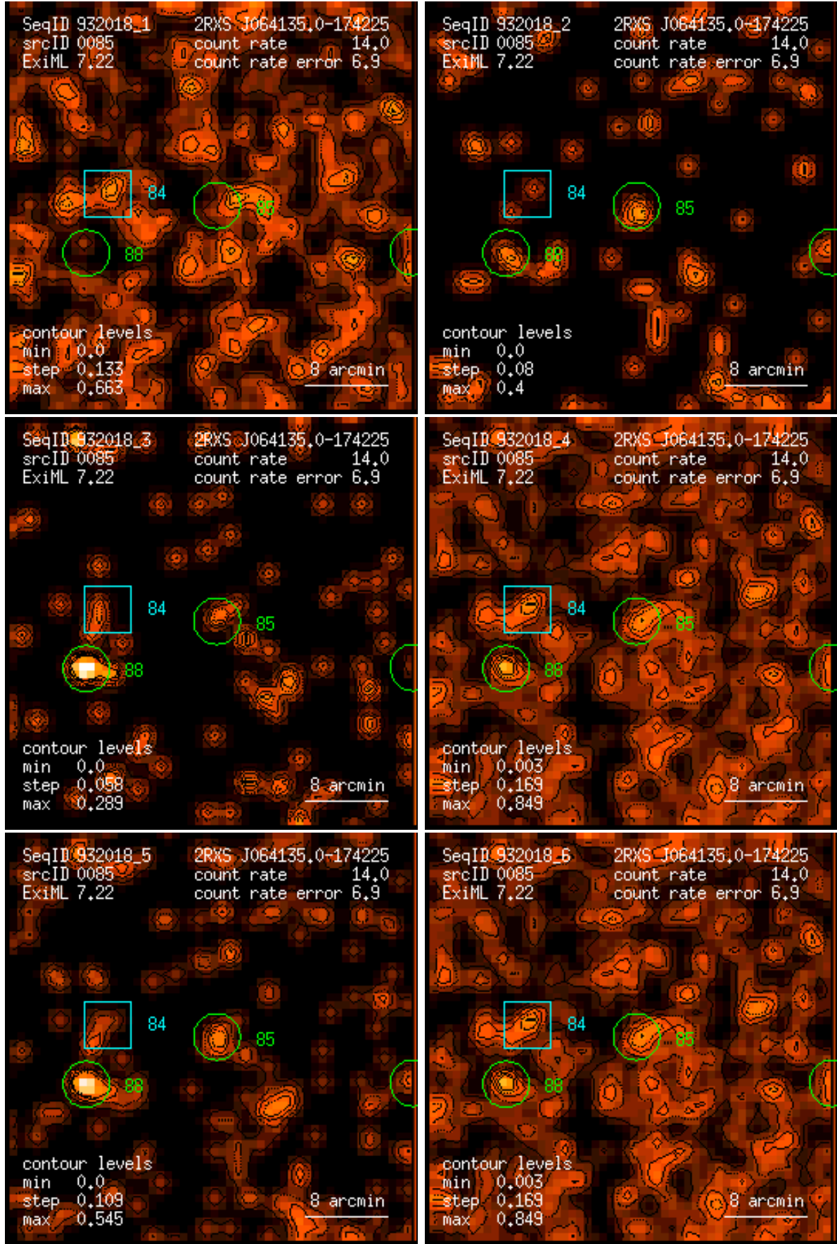
Figure 85: RASS 932018: detection 0085: band rate images, Gaussian filter: (1) PSPC channels 11 – 41, (2) 52 – 90, (3) 91 – 201, (4) 11 – 235, (5) 52 – 201, (6) 11 – 201. Broad band rates in counts/ks. Band rate contour levels in counts/ks/arcmin 2 .
