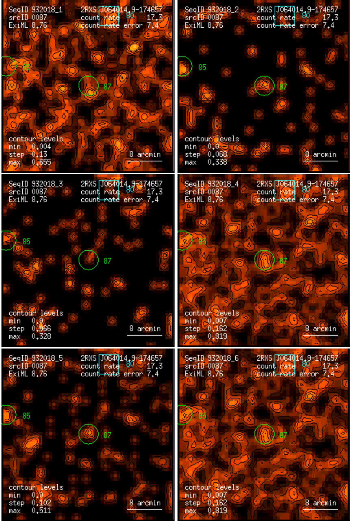
Figure 87: RASS 932018: detection 0087: band rate images, Gaussian filter: (1) PSPC channels 11 – 41, (2) 52 – 90, (3) 91 – 201, (4) 11 – 235, (5) 52 – 201, (6) 11 – 201. Broad band rates in counts/ks. Band rate contour levels in counts/ks/arcmin 2 .
