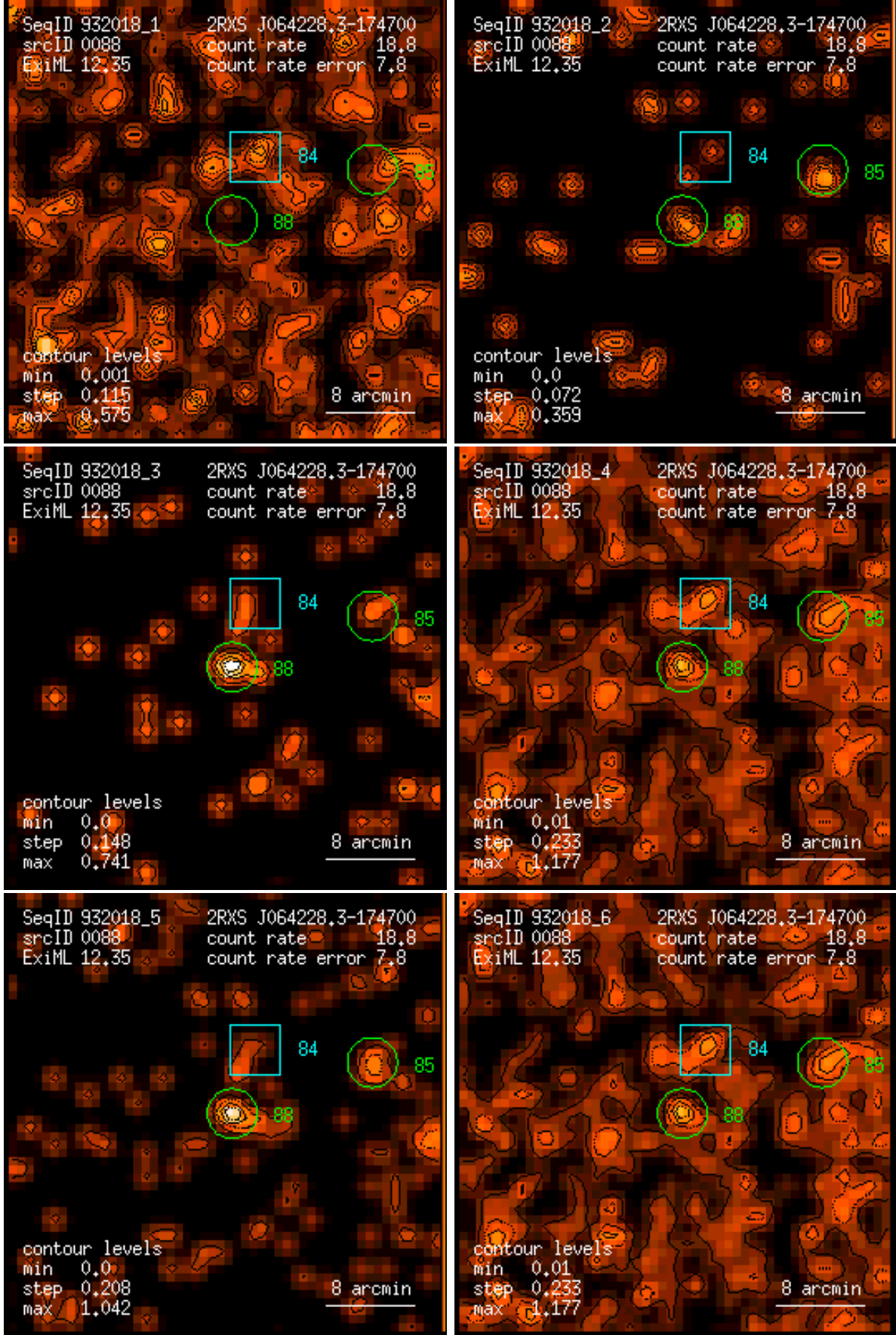
Figure 88: RASS 932018: detection 0088: band rate images, Gaussian filter: (1) PSPC channels 11 – 41, (2) 52 – 90, (3) 91 – 201, (4) 11 – 235, (5) 52 – 201, (6) 11 – 201. Broad band rates in counts/ks. Band rate contour levels in counts/ks/arcmin 2 .
