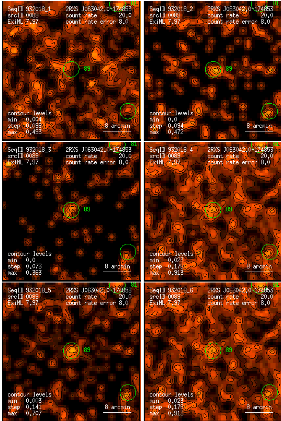
Figure 89: RASS 932018: detection 0089: band rate images, Gaussian filter: (1) PSPC channels 11 – 41, (2) 52 – 90, (3) 91 – 201, (4) 11 – 235, (5) 52 – 201, (6) 11 – 201. Broad band rates in counts/ks. Band rate contour levels in counts/ks/arcmin 2 .
