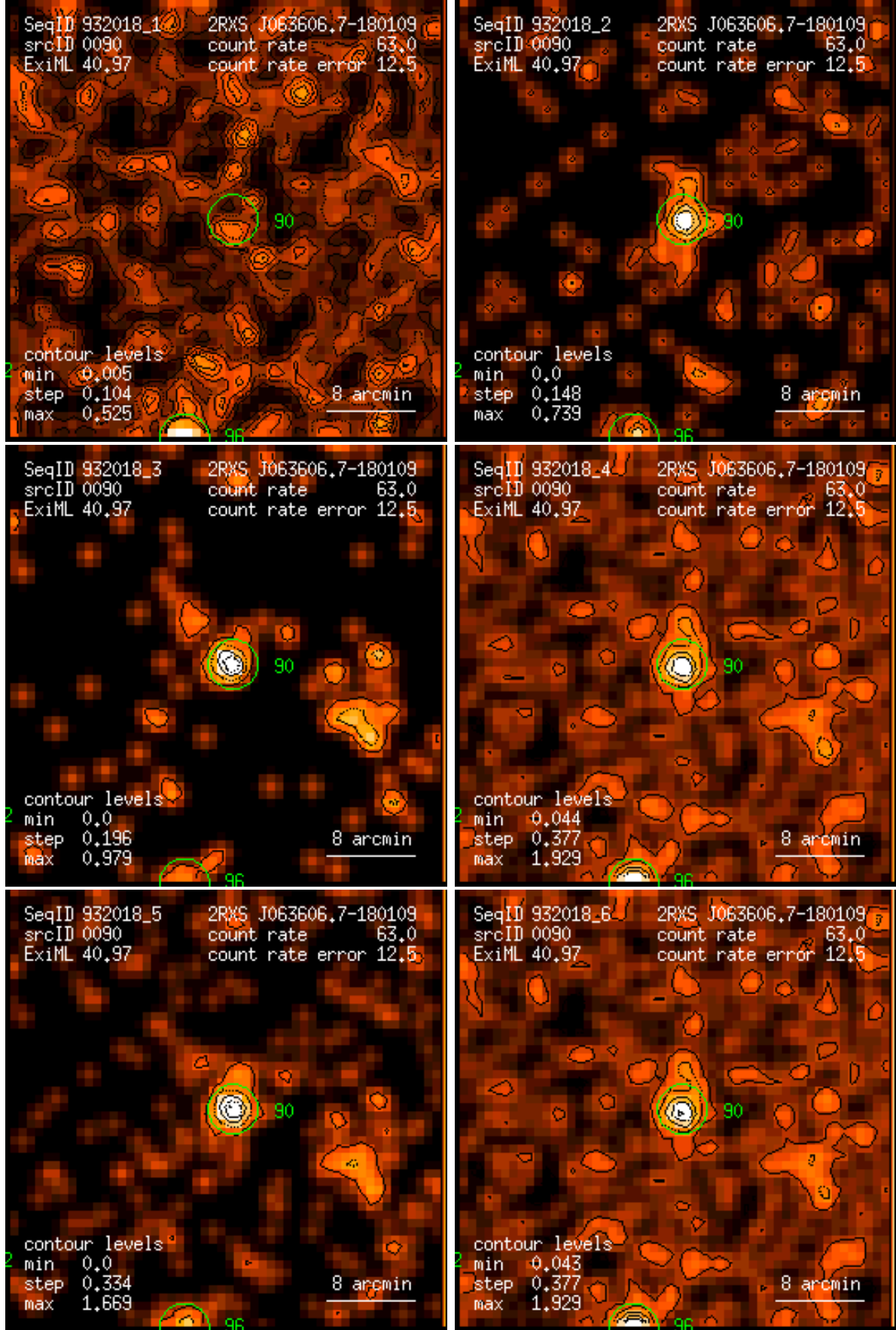
Figure 90: RASS 932018: detection 0090: band rate images, Gaussian filter: (1) PSPC channels 11 – 41, (2) 52 – 90, (3) 91 – 201, (4) 11 – 235, (5) 52 – 201, (6) 11 – 201. Broad band rates in counts/ks. Band rate contour levels in counts/ks/arcmin 2 .
