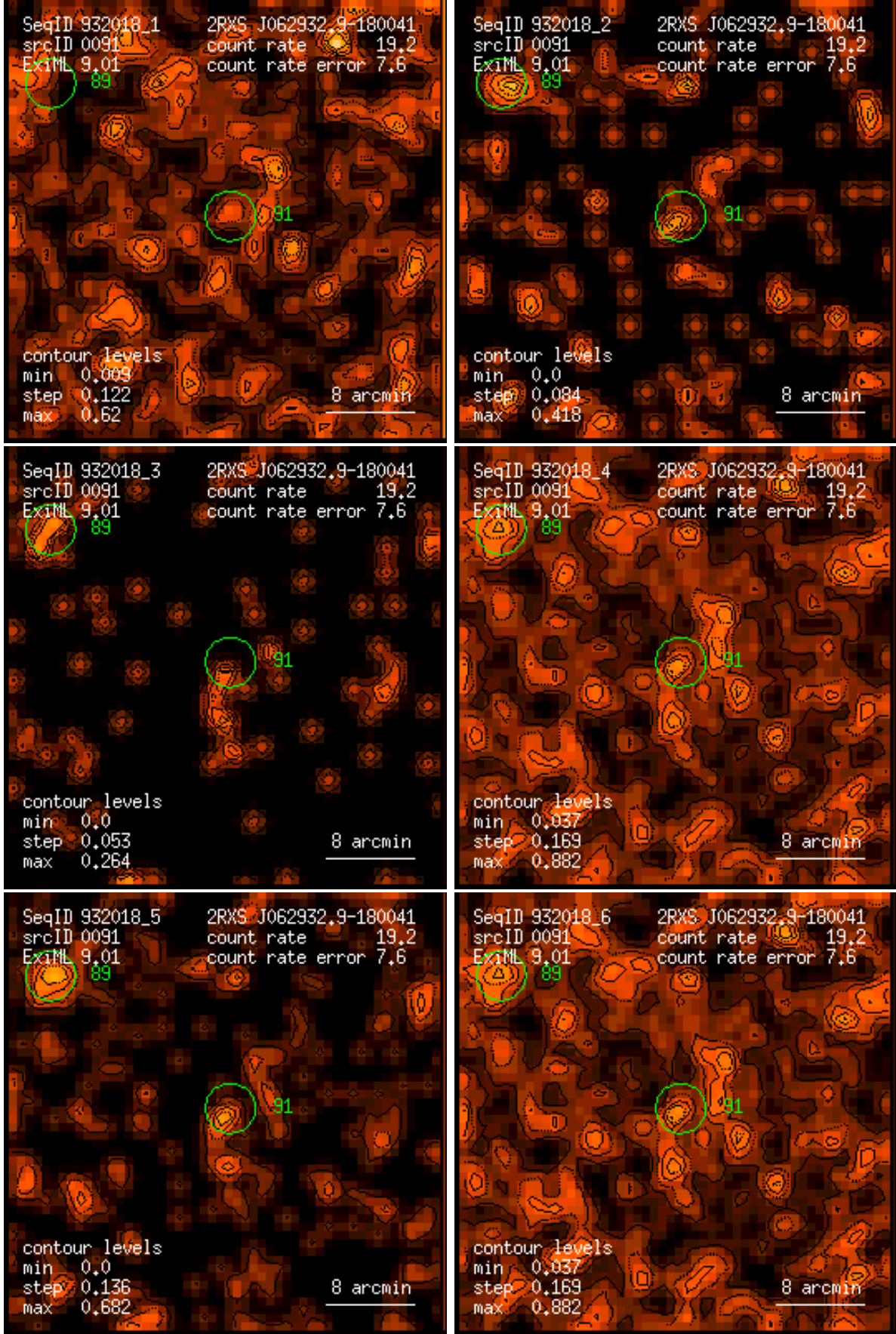
Figure 91: RASS 932018: detection 0091: band rate images, Gaussian filter: (1) PSPC channels 11 – 41, (2) 52 – 90, (3) 91 – 201, (4) 11 – 235, (5) 52 – 201, (6) 11 – 201. Broad band rates in counts/ks. Band rate contour levels in counts/ks/arcmin 2 .
