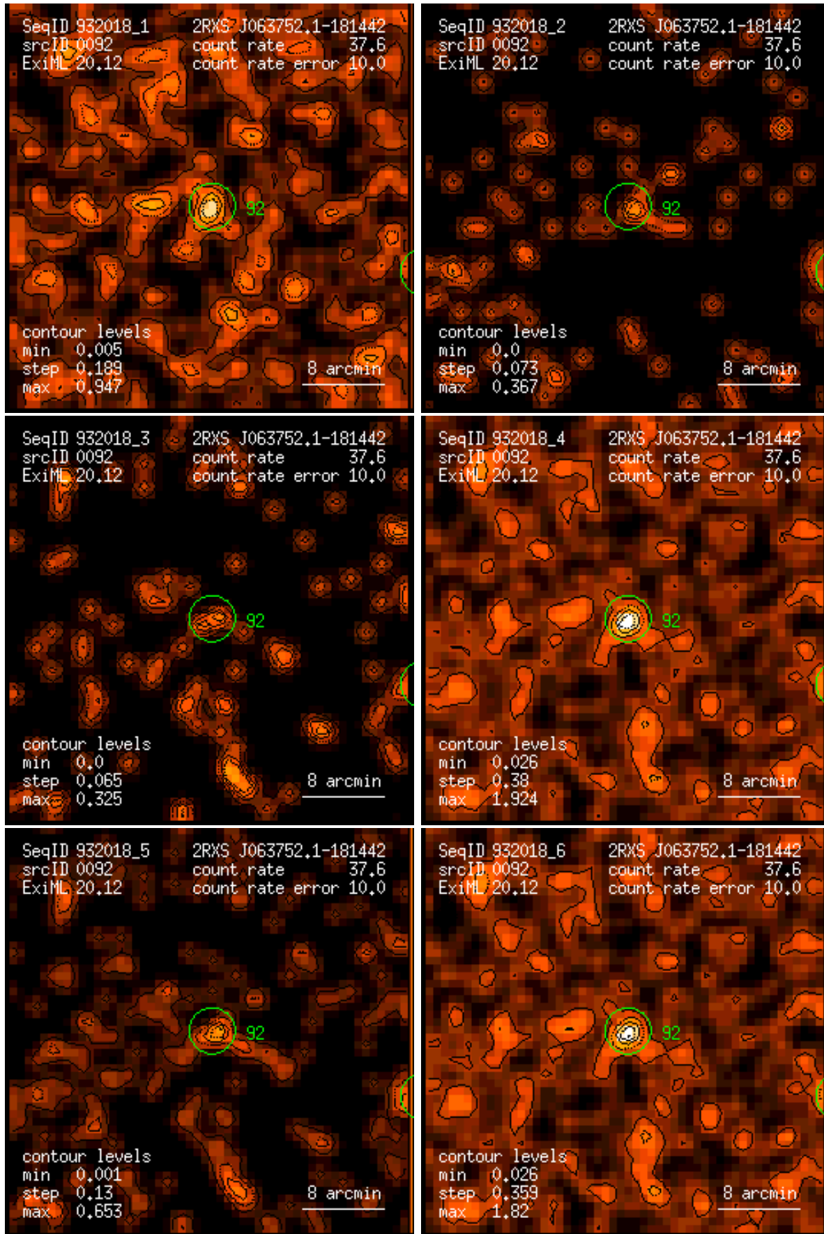
Figure 92: RASS 932018: detection 0092: band rate images, Gaussian filter: (1) PSPC channels 11 – 41, (2) 52 – 90, (3) 91 – 201, (4) 11 – 235, (5) 52 – 201, (6) 11 – 201. Broad band rates in counts/ks. Band rate contour levels in counts/ks/arcmin 2 .
