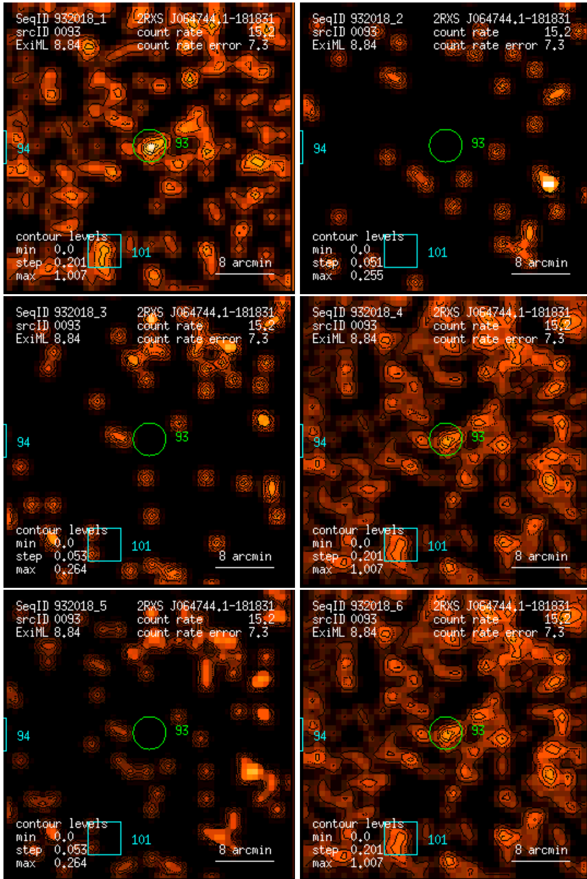
Figure 93: RASS 932018: detection 0093: band rate images, Gaussian filter: (1) PSPC channels 11 – 41, (2) 52 – 90, (3) 91 – 201, (4) 11 – 235, (5) 52 – 201, (6) 11 – 201. Broad band rates in counts/ks. Band rate contour levels in counts/ks/arcmin 2 .
