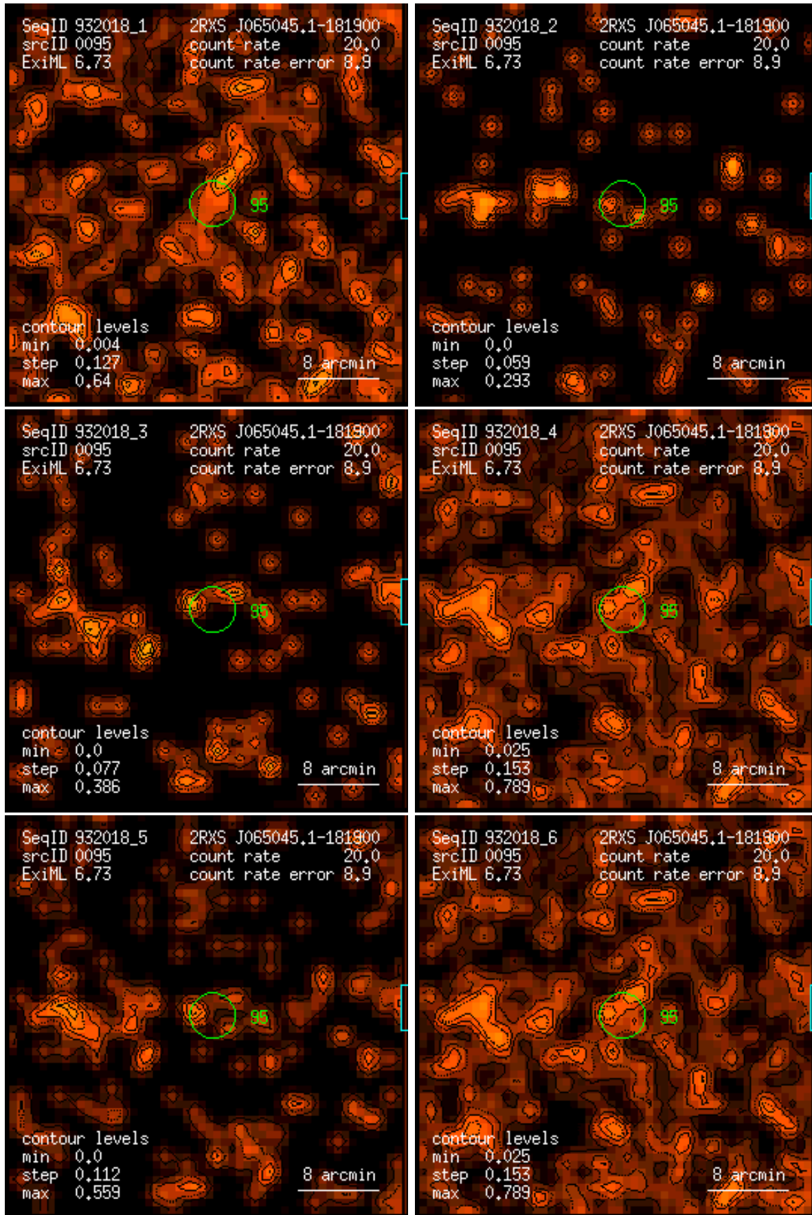
Figure 95: RASS 932018: detection 0095: band rate images, Gaussian filter: (1) PSPC channels 11 – 41, (2) 52 – 90, (3) 91 – 201, (4) 11 – 235, (5) 52 – 201, (6) 11 – 201. Broad band rates in counts/ks. Band rate contour levels in counts/ks/arcmin 2 .
