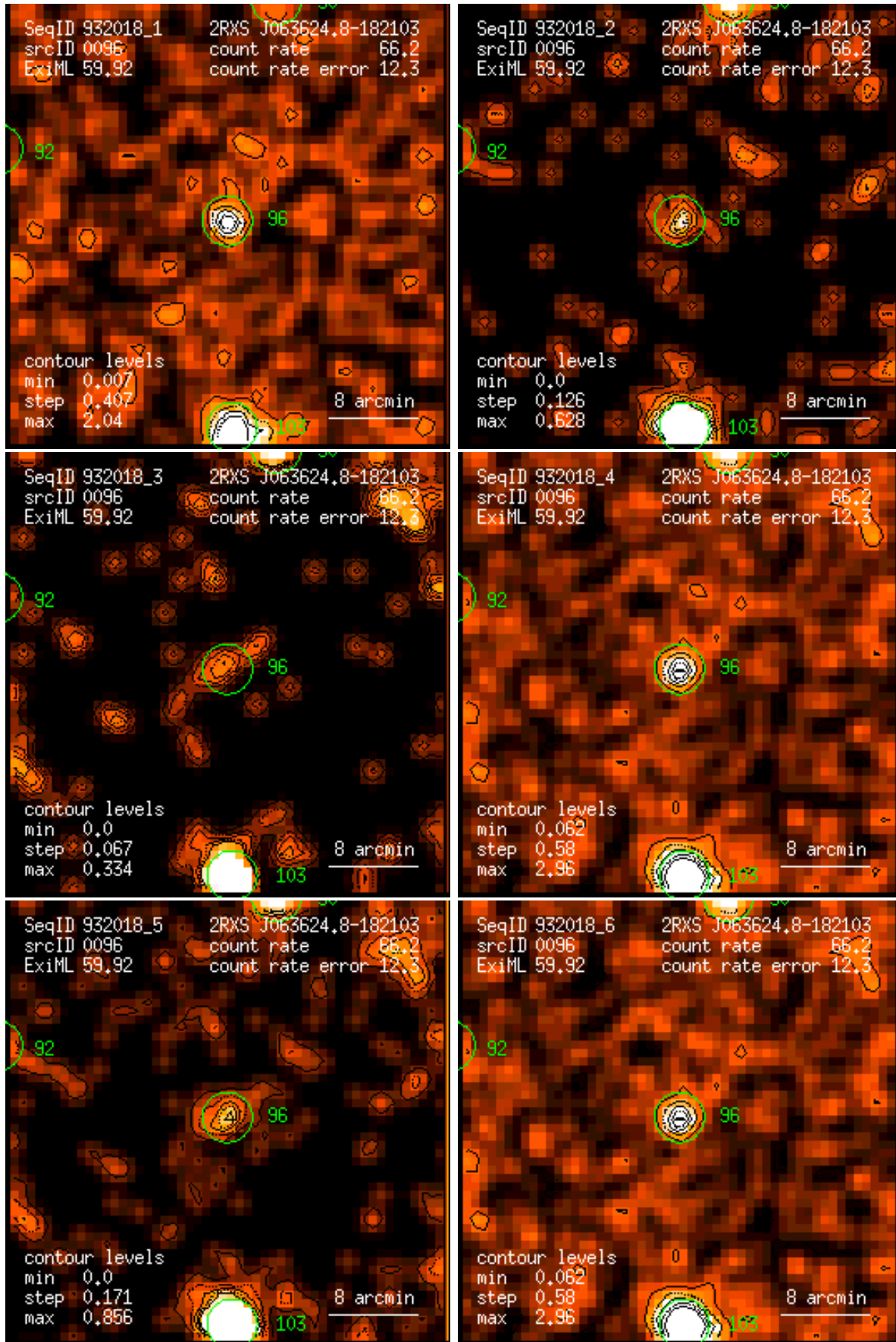
Figure 96: RASS 932018: detection 0096: band rate images, Gaussian filter: (1) PSPC channels 11 – 41, (2) 52 – 90, (3) 91 – 201, (4) 11 – 235, (5) 52 – 201, (6) 11 – 201. Broad band rates in counts/ks. Band rate contour levels in counts/ks/arcmin 2 .
