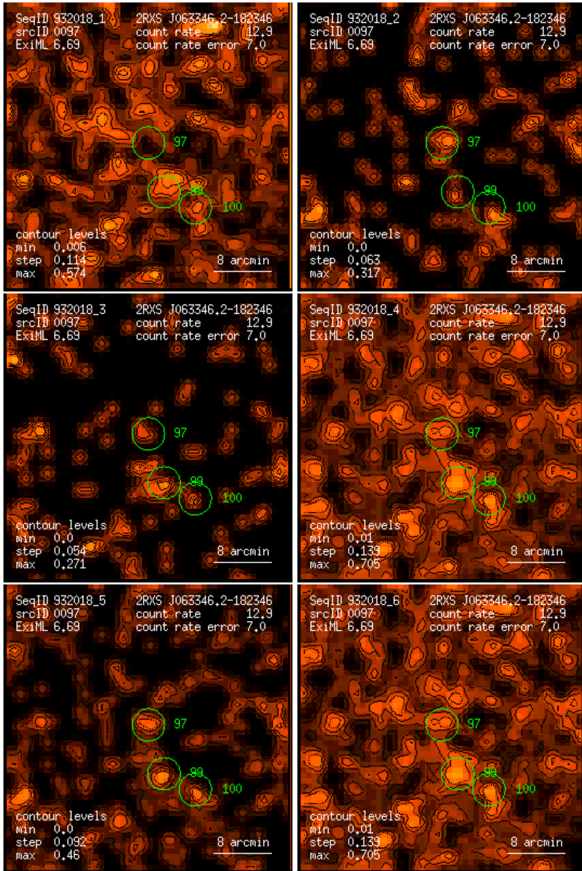
Figure 97: RASS 932018: detection 0097: band rate images, Gaussian filter: (1) PSPC channels 11 – 41, (2) 52 – 90, (3) 91 – 201, (4) 11 – 235, (5) 52 – 201, (6) 11 – 201. Broad band rates in counts/ks. Band rate contour levels in counts/ks/arcmin 2 .
