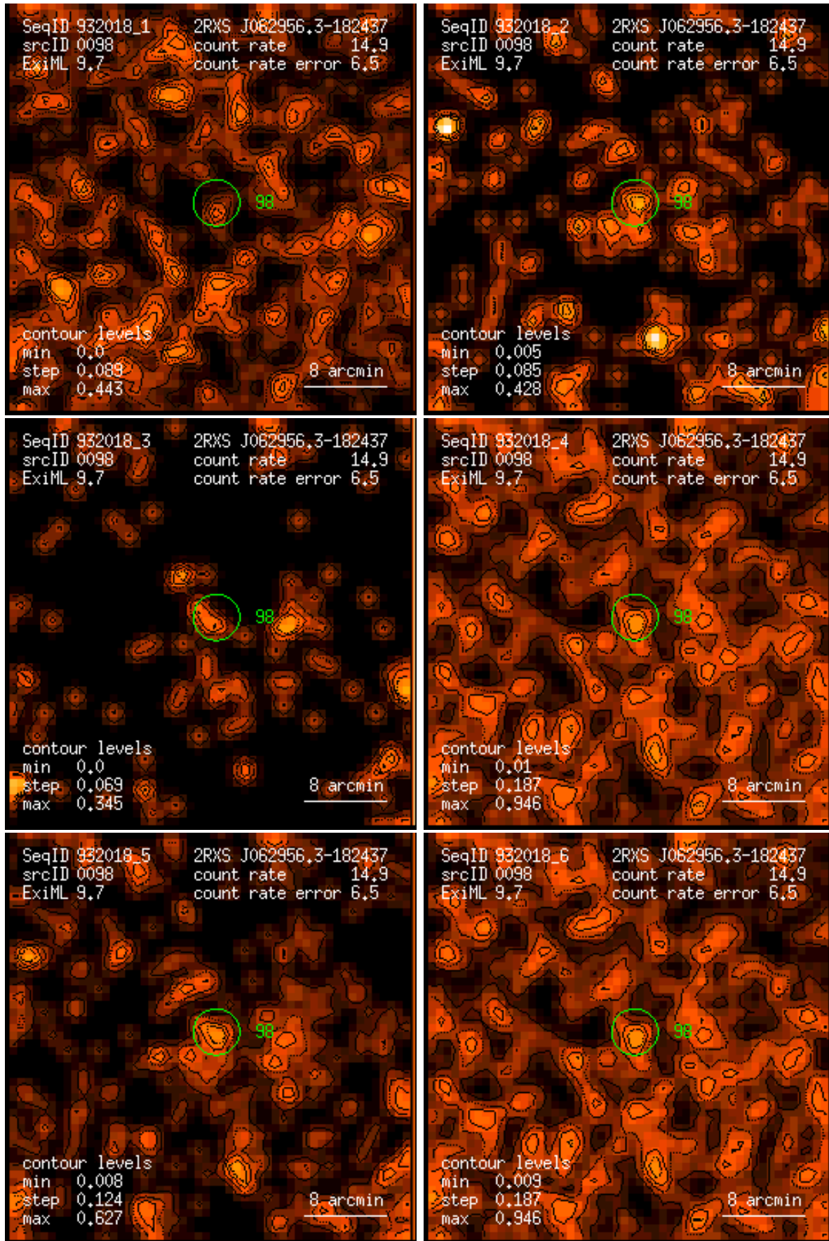
Figure 98: RASS 932018: detection 0098: band rate images, Gaussian filter: (1) PSPC channels 11 – 41, (2) 52 – 90, (3) 91 – 201, (4) 11 – 235, (5) 52 – 201, (6) 11 – 201. Broad band rates in counts/ks. Band rate contour levels in counts/ks/arcmin 2 .
