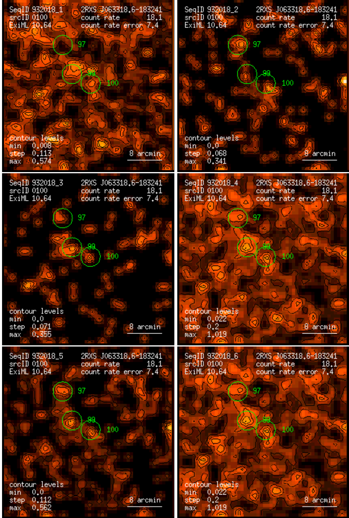
Figure 100: RASS 932018: detection 0100: band rate images, Gaussian filter: (1) PSPC channels 11 – 41, (2) 52 – 90, (3) 91 – 201, (4) 11 – 235, (5) 52 – 201, (6) 11 – 201. Broad band rates in counts/ks. Band rate contour levels in counts/ks/arcmin 2 .
