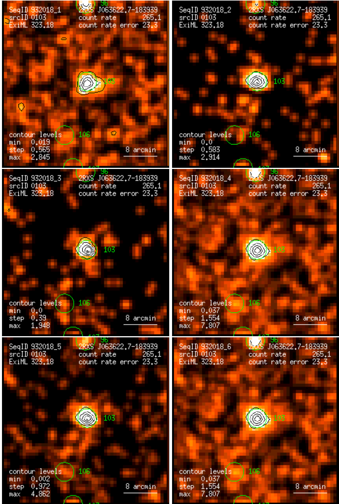
Figure 103: RASS 932018: detection 0103: band rate images, Gaussian filter: (1) PSPC channels 11 – 41, (2) 52 – 90, (3) 91 – 201, (4) 11 – 235, (5) 52 – 201, (6) 11 – 201. Broad band rates in counts/ks. Band rate contour levels in counts/ks/arcmin 2 .
