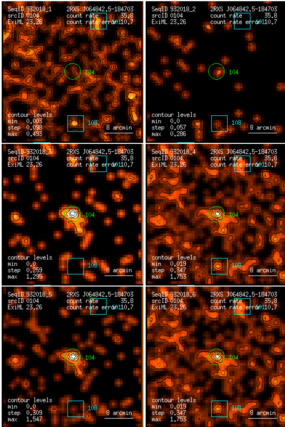
Figure 104: RASS 932018: detection 0104: band rate images, Gaussian filter: (1) PSPC channels 11 – 41, (2) 52 – 90, (3) 91 – 201, (4) 11 – 235, (5) 52 – 201, (6) 11 – 201. Broad band rates in counts/ks. Band rate contour levels in counts/ks/arcmin 2 .
