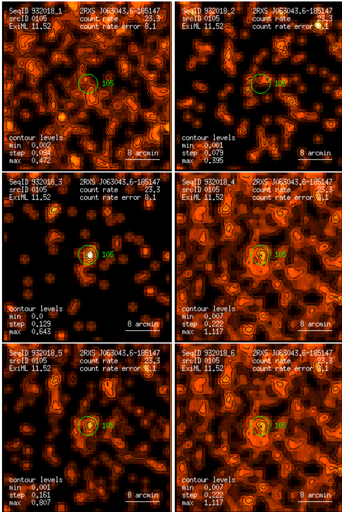
Figure 105: RASS 932018: detection 0105: band rate images, Gaussian filter: (1) PSPC channels 11 – 41, (2) 52 – 90, (3) 91 – 201, (4) 11 – 235, (5) 52 – 201, (6) 11 – 201. Broad band rates in counts/ks. Band rate contour levels in counts/ks/arcmin 2 .
