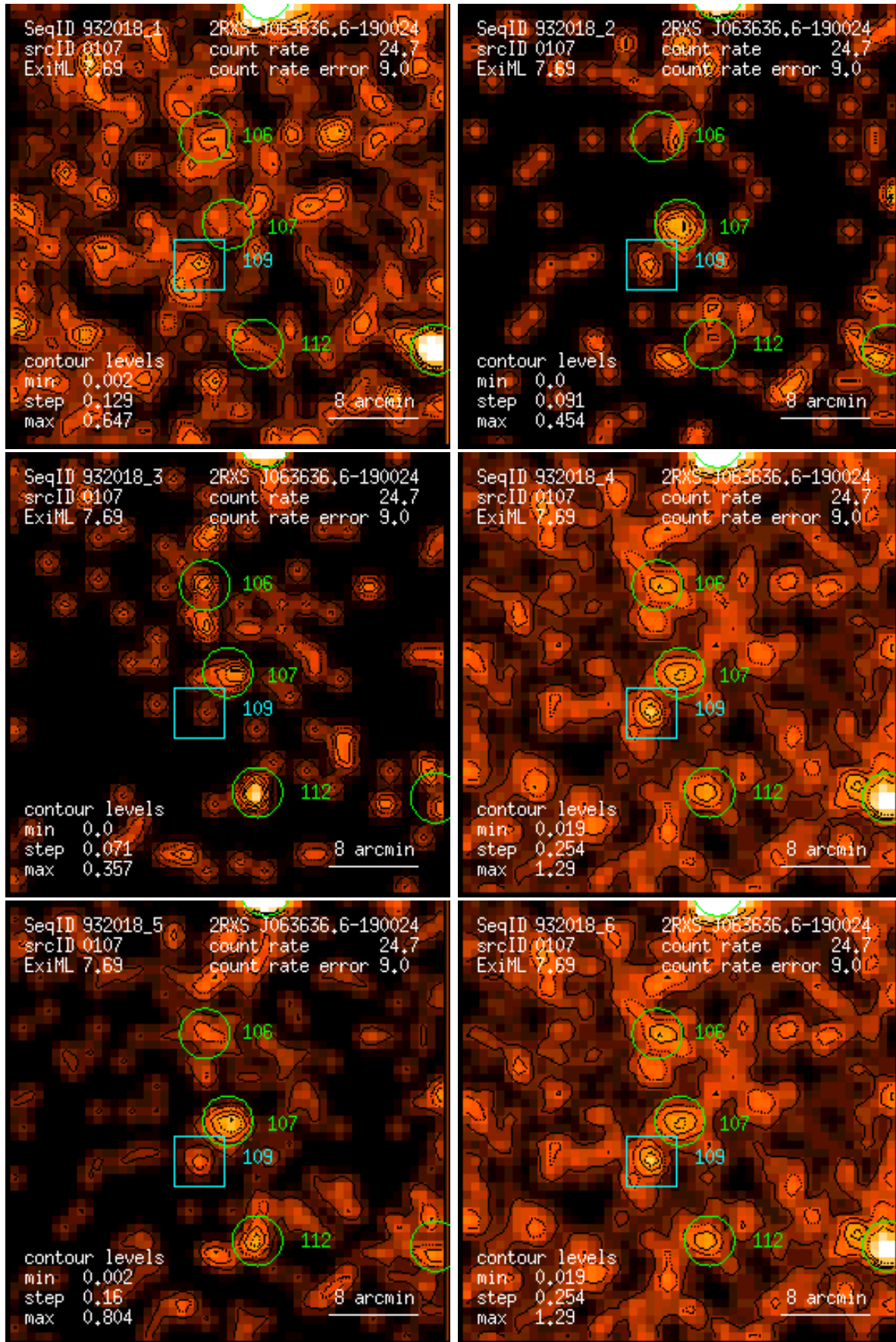
Figure 107: RASS 932018: detection 0107: band rate images, Gaussian filter: (1) PSPC channels 11 – 41, (2) 52 – 90, (3) 91 – 201, (4) 11 – 235, (5) 52 – 201, (6) 11 – 201. Broad band rates in counts/ks. Band rate contour levels in counts/ks/arcmin 2 .
