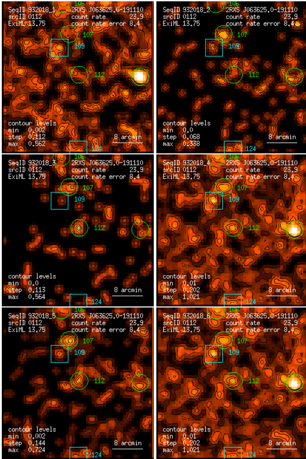
Figure 112: RASS 932018: detection 0112: band rate images, Gaussian filter: (1) PSPC channels 11 – 41, (2) 52 – 90, (3) 91 – 201, (4) 11 – 235, (5) 52 – 201, (6) 11 – 201. Broad band rates in counts/ks. Band rate contour levels in counts/ks/arcmin 2 .
