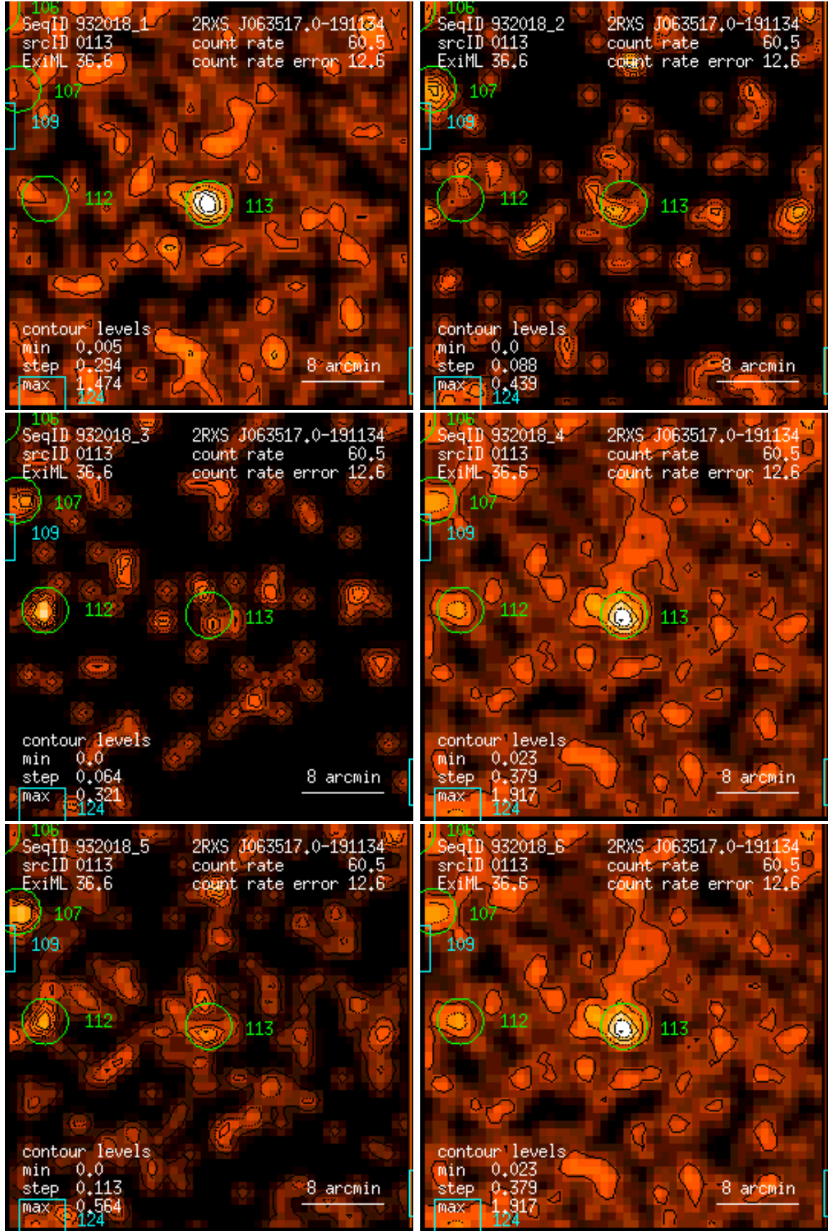
Figure 113: RASS 932018: detection 0113: band rate images, Gaussian filter: (1) PSPC channels 11 – 41, (2) 52 – 90, (3) 91 – 201, (4) 11 – 235, (5) 52 – 201, (6) 11 – 201. Broad band rates in counts/ks. Band rate contour levels in counts/ks/arcmin 2 .
