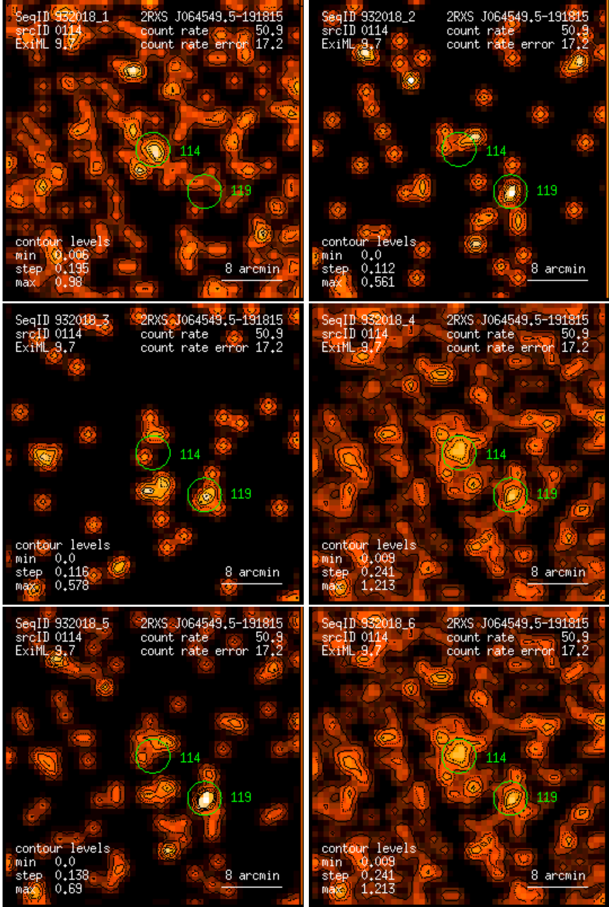
Figure 114: RASS 932018: detection 0114: band rate images, Gaussian filter: (1) PSPC channels 11 – 41, (2) 52 – 90, (3) 91 – 201, (4) 11 – 235, (5) 52 – 201, (6) 11 – 201. Broad band rates in counts/ks. Band rate contour levels in counts/ks/arcmin 2 .
