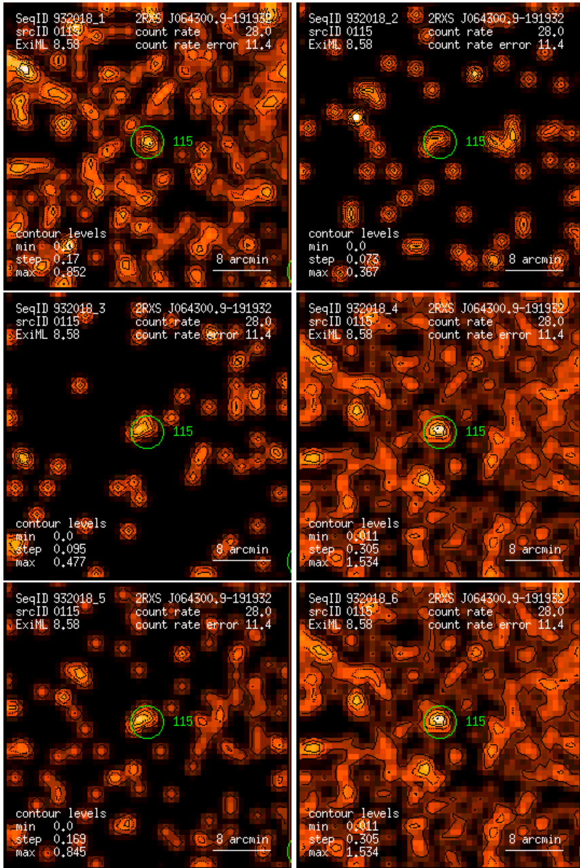
Figure 115: RASS 932018: detection 0115: band rate images, Gaussian filter: (1) PSPC channels 11 – 41, (2) 52 – 90, (3) 91 – 201, (4) 11 – 235, (5) 52 – 201, (6) 11 – 201. Broad band rates in counts/ks. Band rate contour levels in counts/ks/arcmin 2 .
