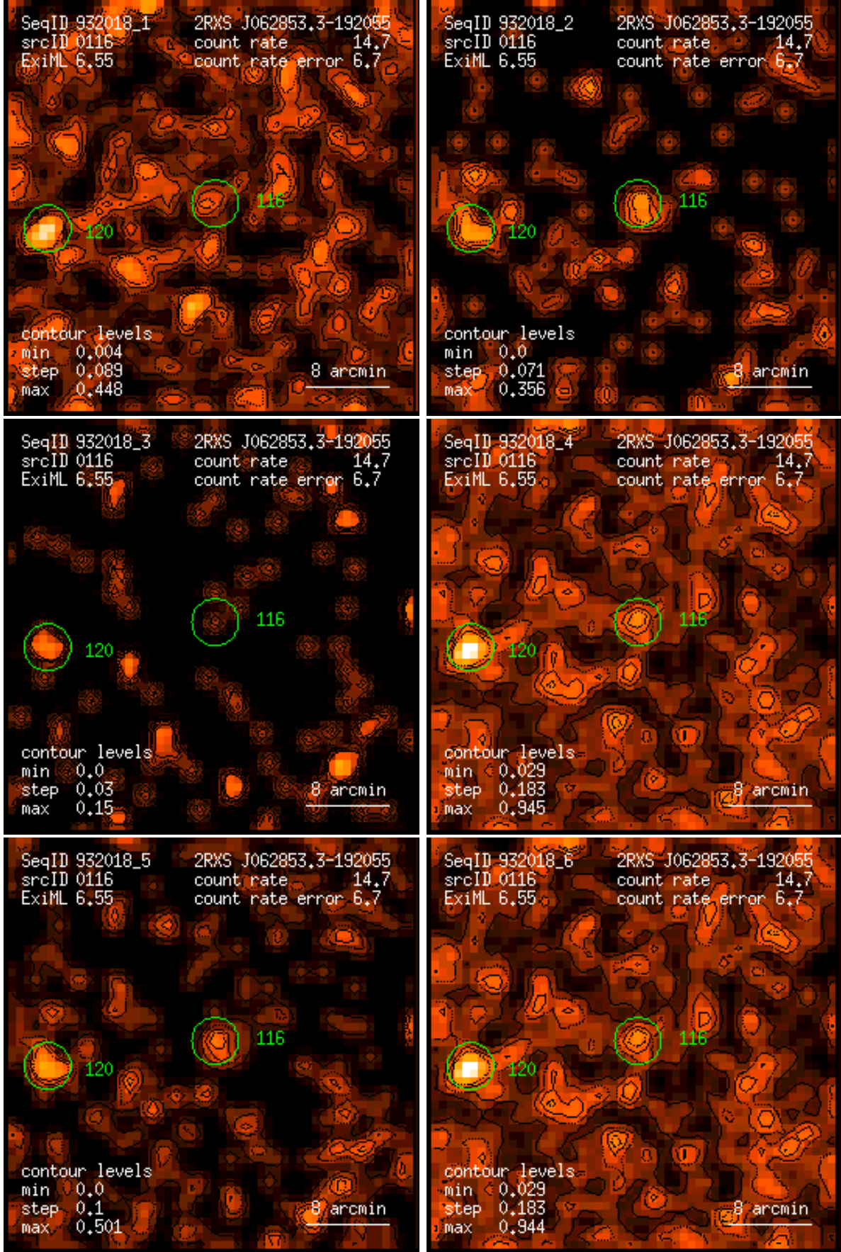
Figure 116: RASS 932018: detection 0116: band rate images, Gaussian filter: (1) PSPC channels 11 – 41, (2) 52 – 90, (3) 91 – 201, (4) 11 – 235, (5) 52 – 201, (6) 11 – 201. Broad band rates in counts/ks. Band rate contour levels in counts/ks/arcmin 2 .
