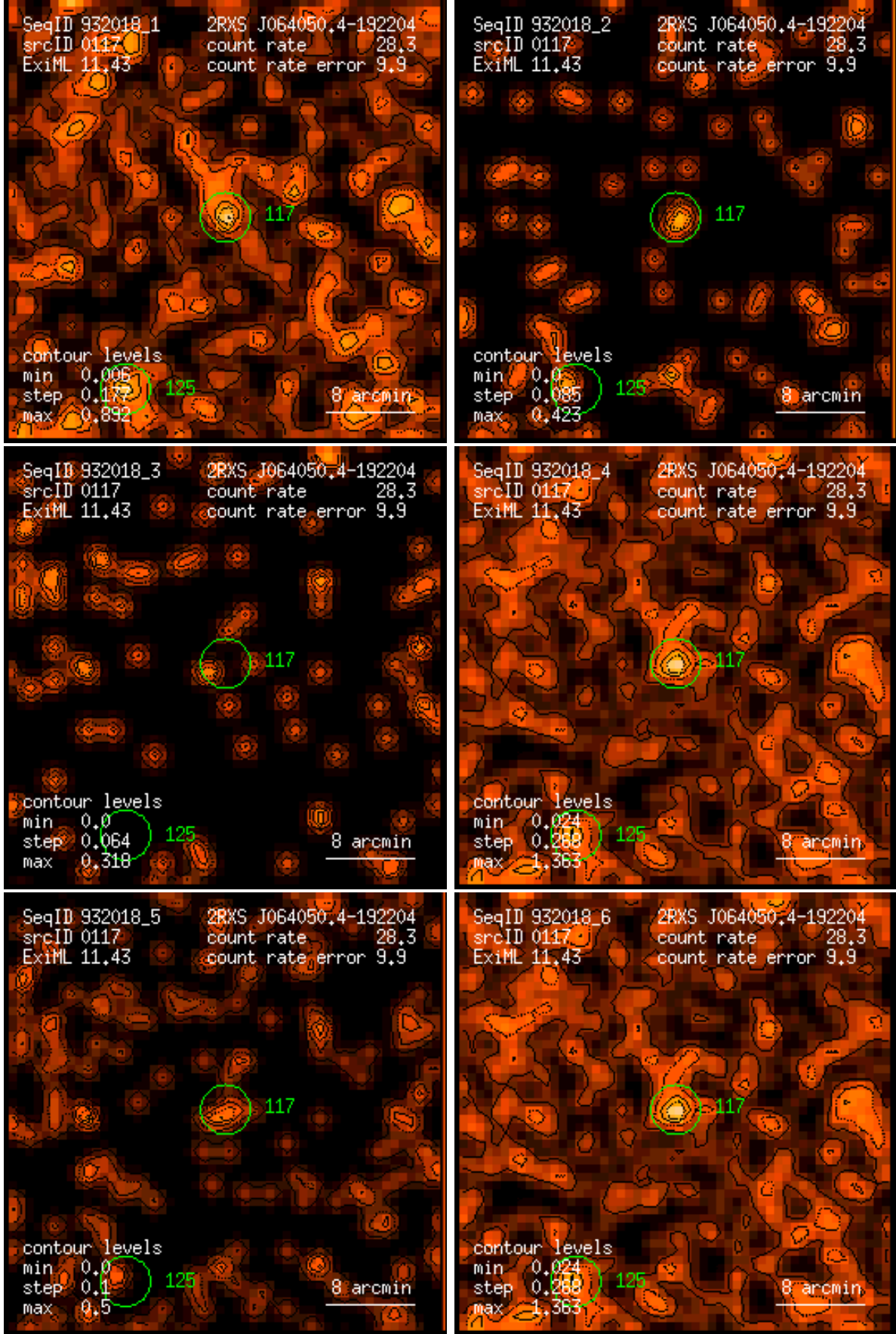
Figure 117: RASS 932018: detection 0117: band rate images, Gaussian filter: (1) PSPC channels 11 – 41, (2) 52 – 90, (3) 91 – 201, (4) 11 – 235, (5) 52 – 201, (6) 11 – 201. Broad band rates in counts/ks. Band rate contour levels in counts/ks/arcmin 2 .
