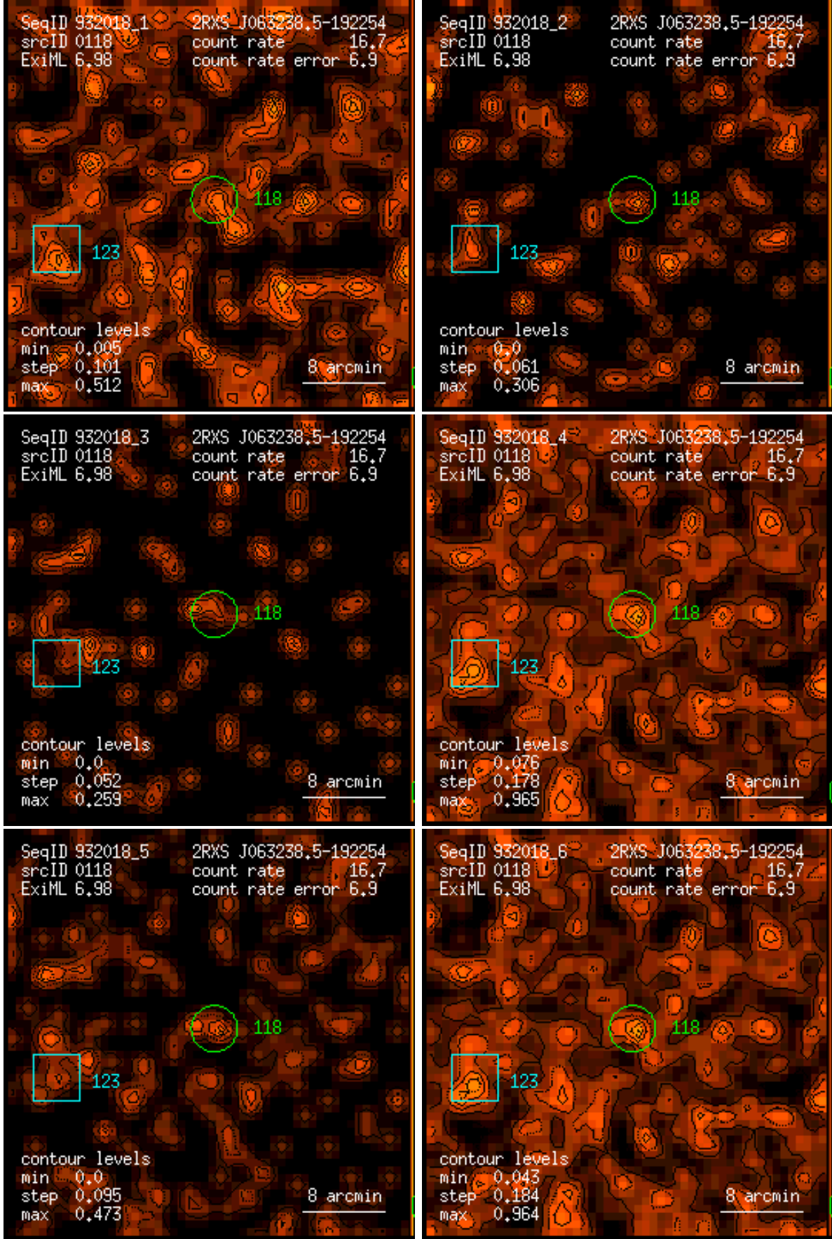
Figure 118: RASS 932018: detection 0118: band rate images, Gaussian filter: (1) PSPC channels 11 – 41, (2) 52 – 90, (3) 91 – 201, (4) 11 – 235, (5) 52 – 201, (6) 11 – 201. Broad band rates in counts/ks. Band rate contour levels in counts/ks/arcmin 2 .
