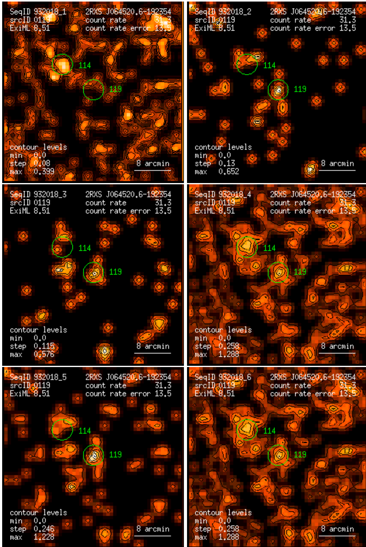
Figure 119: RASS 932018: detection 0119: band rate images, Gaussian filter: (1) PSPC channels 11 – 41, (2) 52 – 90, (3) 91 – 201, (4) 11 – 235, (5) 52 – 201, (6) 11 – 201. Broad band rates in counts/ks. Band rate contour levels in counts/ks/arcmin 2 .
