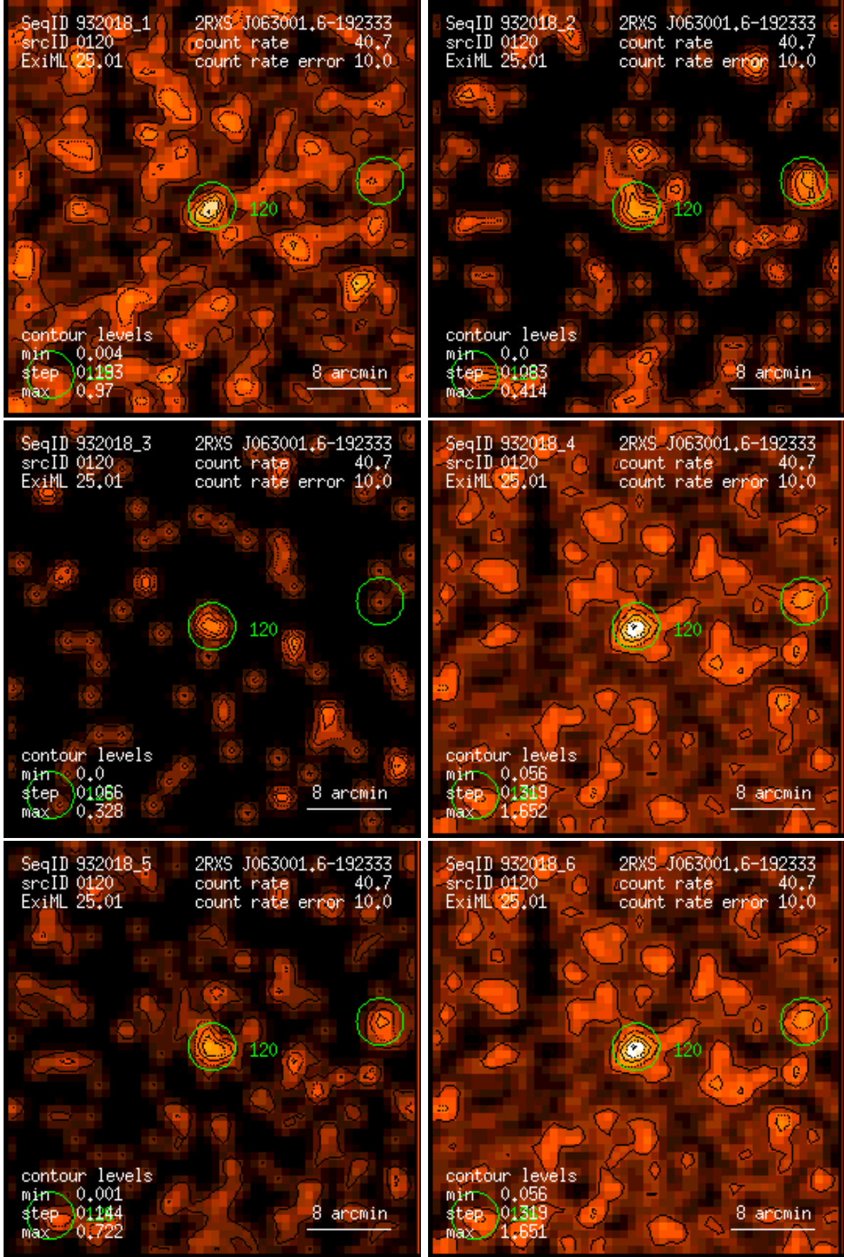
Figure 120: RASS 932018: detection 0120: band rate images, Gaussian filter: (1) PSPC channels 11 – 41, (2) 52 – 90, (3) 91 – 201, (4) 11 – 235, (5) 52 – 201, (6) 11 – 201. Broad band rates in counts/ks. Band rate contour levels in counts/ks/arcmin 2 .
