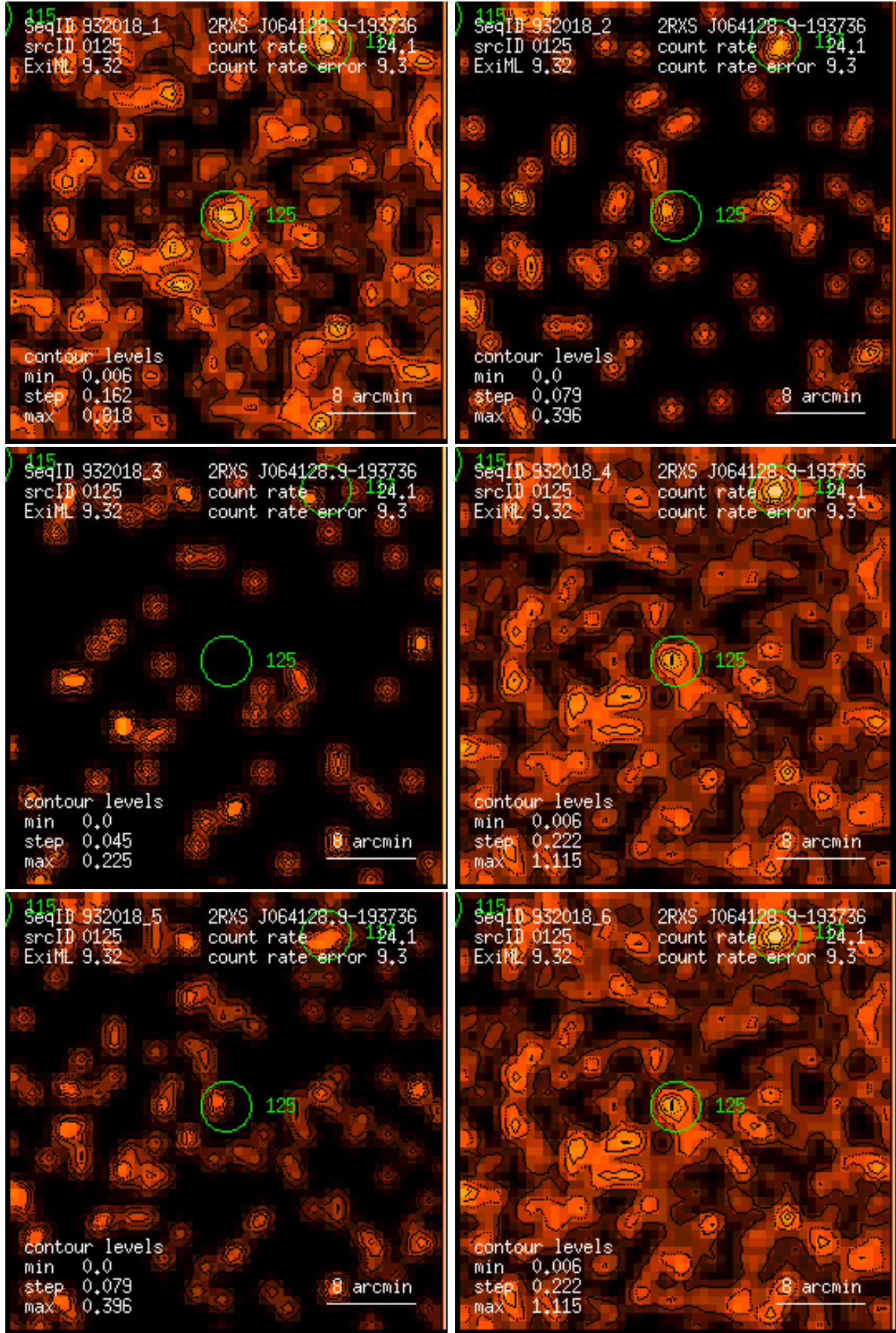
Figure 125: RASS 932018: detection 0125: band rate images, Gaussian filter: (1) PSPC channels 11 – 41, (2) 52 – 90, (3) 91 – 201, (4) 11 – 235, (5) 52 – 201, (6) 11 – 201. Broad band rates in counts/ks. Band rate contour levels in counts/ks/arcmin 2 .
