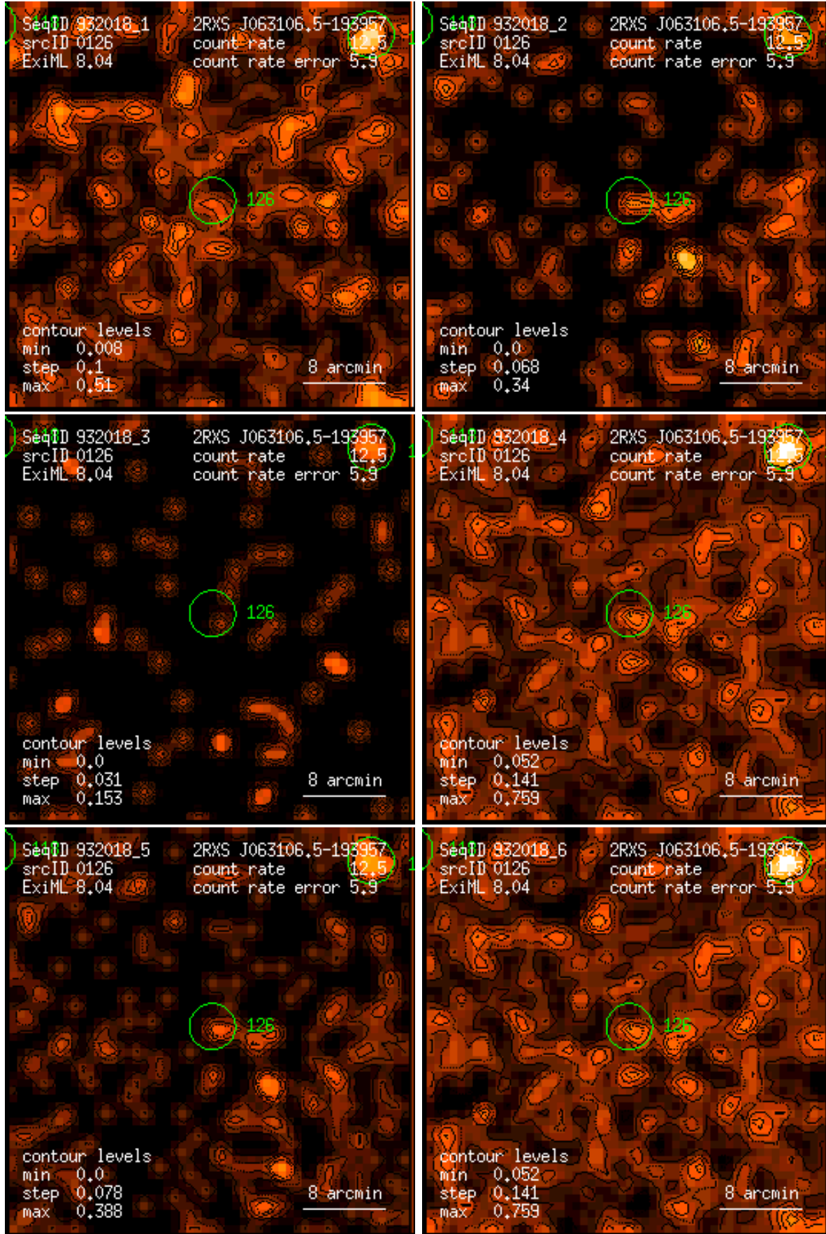
Figure 126: RASS 932018: detection 0126: band rate images, Gaussian filter: (1) PSPC channels 11 – 41, (2) 52 – 90, (3) 91 – 201, (4) 11 – 235, (5) 52 – 201, (6) 11 – 201. Broad band rates in counts/ks. Band rate contour levels in counts/ks/arcmin 2 .
