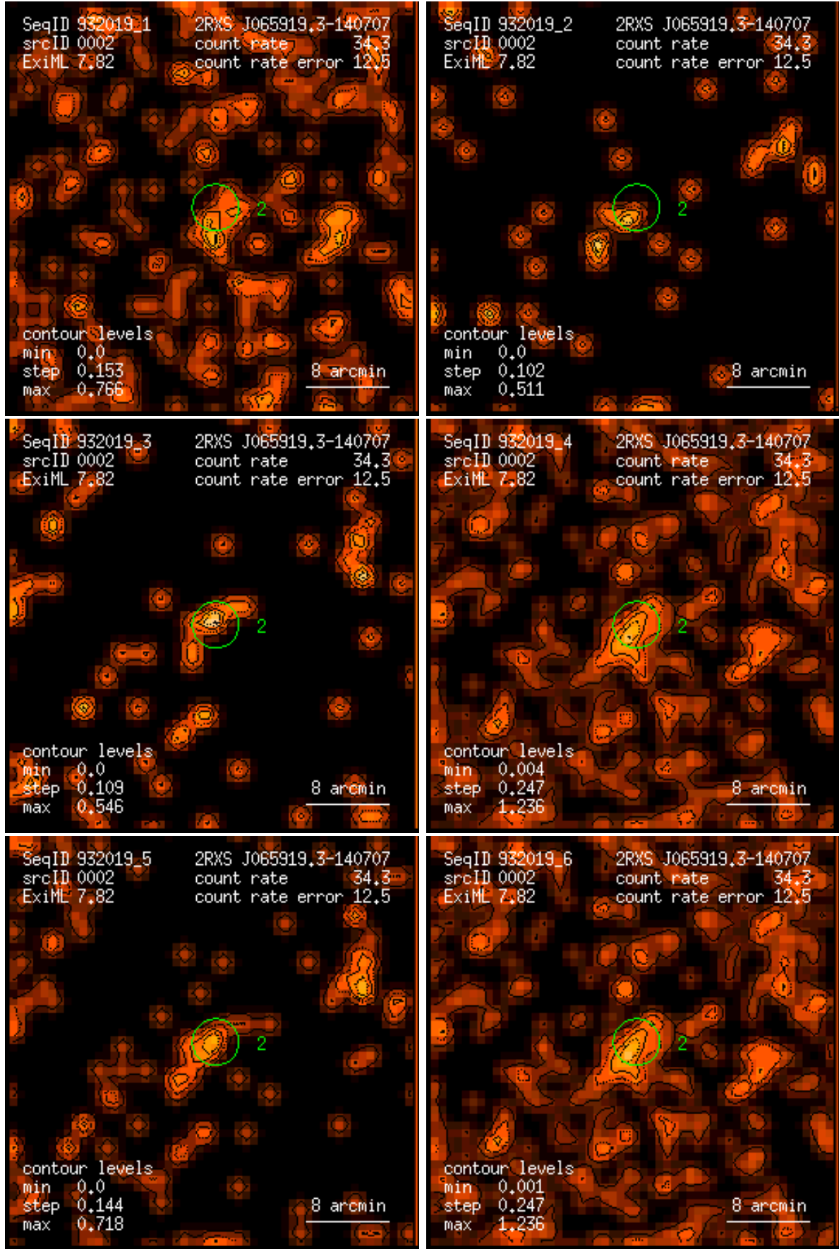
Figure 2: RASS 932019: detection 0002: band rate images, Gaussian filter: (1) PSPC channels 11 – 41, (2) 52 – 90, (3) 91 – 201, (4) 11 – 235, (5) 52 – 201, (6) 11 – 201. Broad band rates in counts/ks. Band rate contour levels in counts/ks/arcmin 2 .
