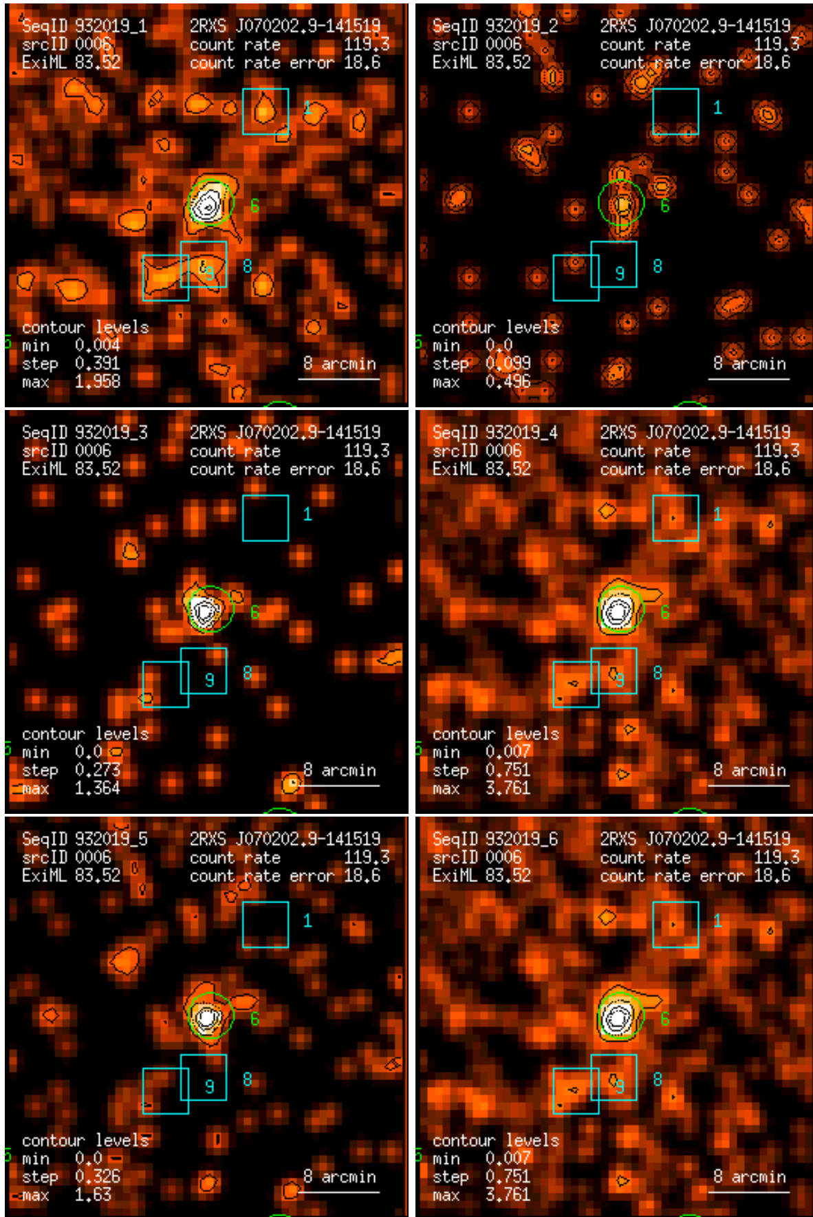
Figure 6: RASS 932019: detection 0006: band rate images, Gaussian filter: (1) PSPC channels 11 – 41, (2) 52 – 90, (3) 91 – 201, (4) 11 – 235, (5) 52 – 201, (6) 11 – 201. Broad band rates in counts/ks. Band rate contour levels in counts/ks/arcmin 2 .
