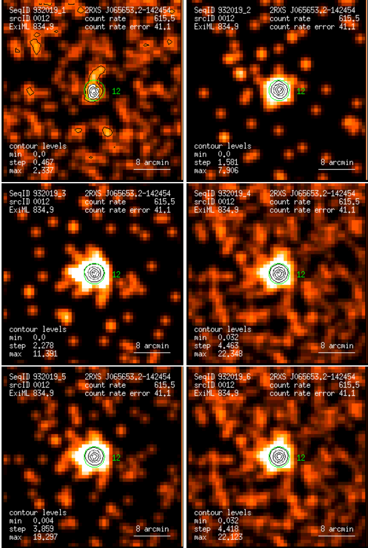
Figure 12: RASS 932019: detection 0012: band rate images, Gaussian filter: (1) PSPC channels 11 – 41, (2) 52 – 90, (3) 91 – 201, (4) 11 – 235, (5) 52 – 201, (6) 11 – 201. Broad band rates in counts/ks. Band rate contour levels in counts/ks/arcmin 2 .
