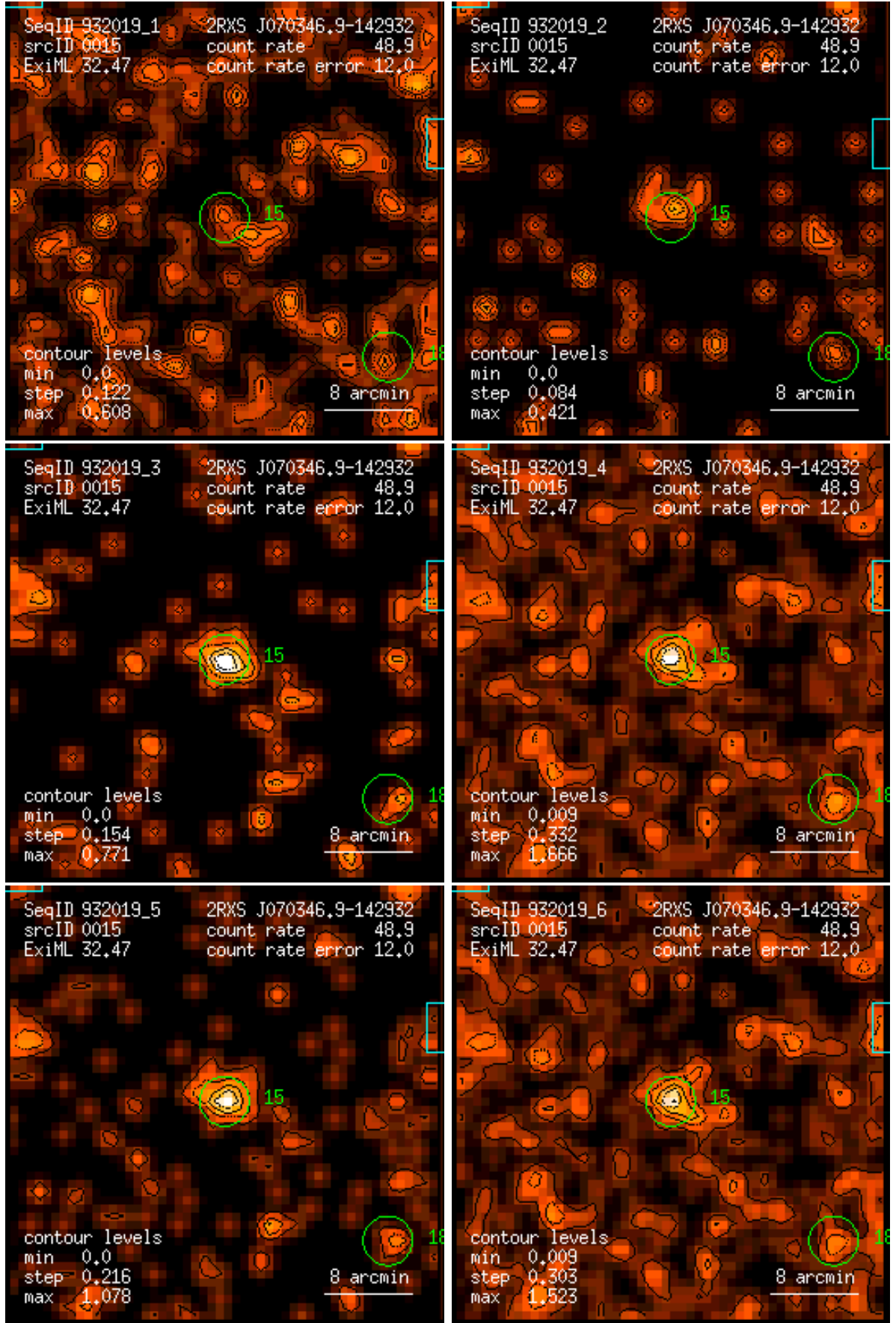
Figure 15: RASS 932019: detection 0015: band rate images, Gaussian filter: (1) PSPC channels 11 – 41, (2) 52 – 90, (3) 91 – 201, (4) 11 – 235, (5) 52 – 201, (6) 11 – 201. Broad band rates in counts/ks. Band rate contour levels in counts/ks/arcmin 2 .
