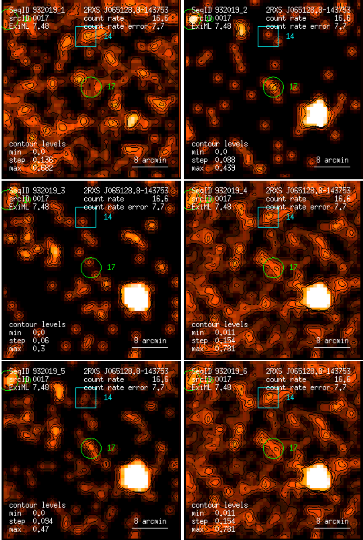
Figure 17: RASS 932019: detection 0017: band rate images, Gaussian filter: (1) PSPC channels 11 – 41, (2) 52 – 90, (3) 91 – 201, (4) 11 – 235, (5) 52 – 201, (6) 11 – 201. Broad band rates in counts/ks. Band rate contour levels in counts/ks/arcmin 2 .
