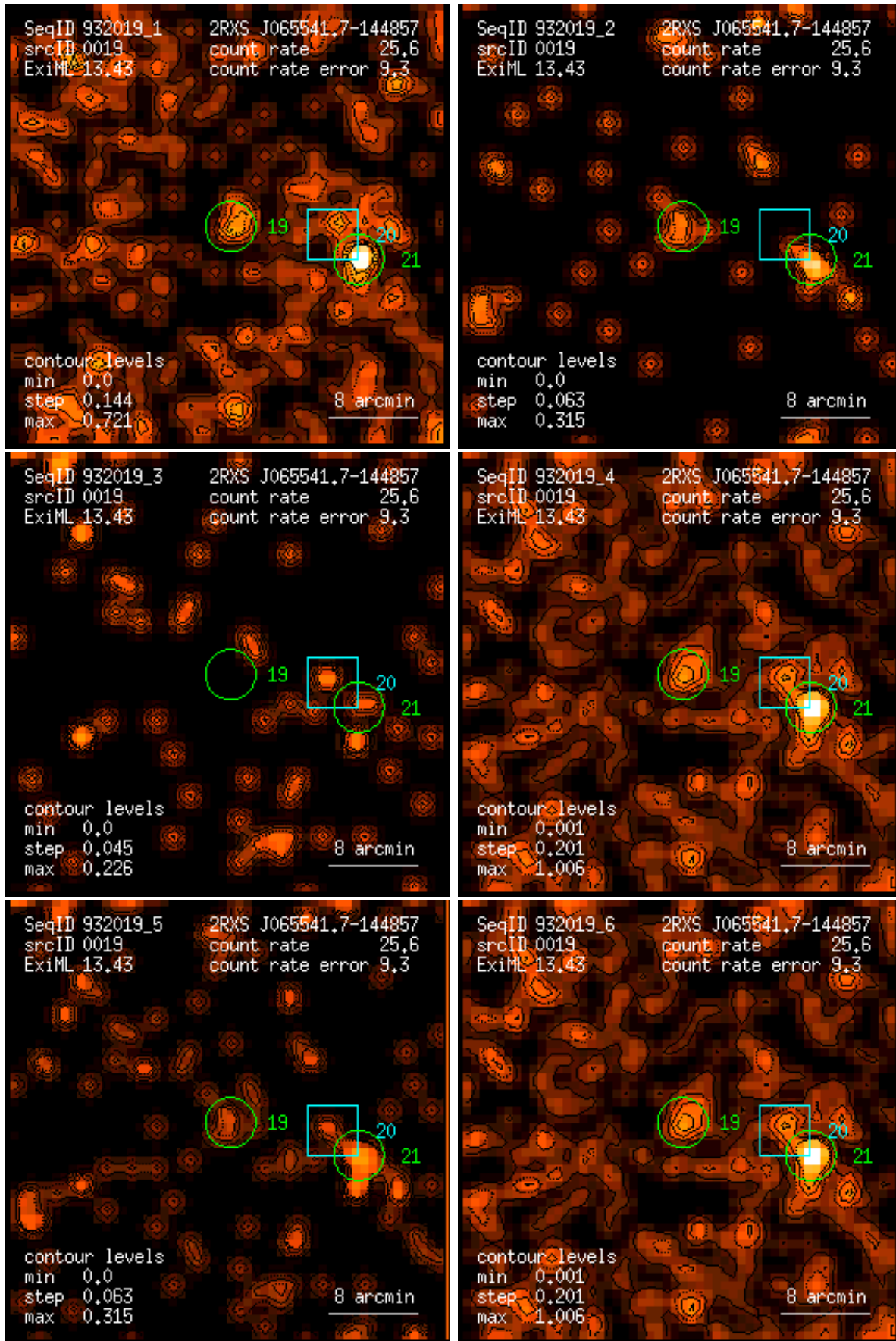
Figure 19: RASS 932019: detection 0019: band rate images, Gaussian filter: (1) PSPC channels 11 – 41, (2) 52 – 90, (3) 91 – 201, (4) 11 – 235, (5) 52 – 201, (6) 11 – 201. Broad band rates in counts/ks. Band rate contour levels in counts/ks/arcmin 2 .
