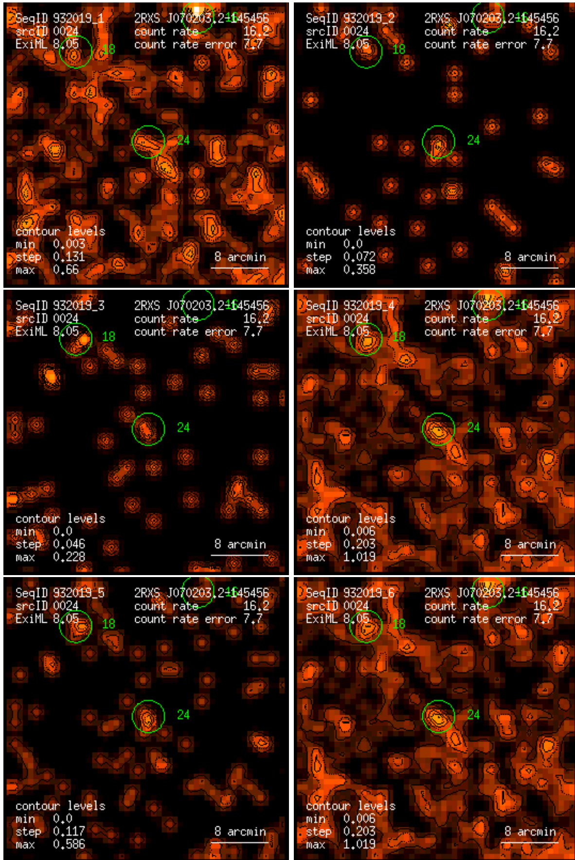
Figure 24: RASS 932019: detection 0024: band rate images, Gaussian filter: (1) PSPC channels 11 – 41, (2) 52 – 90, (3) 91 – 201, (4) 11 – 235, (5) 52 – 201, (6) 11 – 201. Broad band rates in counts/ks. Band rate contour levels in counts/ks/arcmin 2 .
