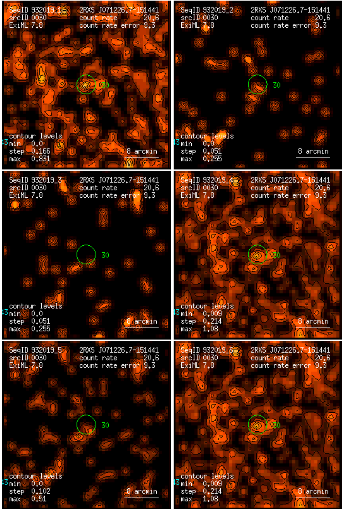
Figure 30: RASS 932019: detection 0030: band rate images, Gaussian filter: (1) PSPC channels 11 – 41, (2) 52 – 90, (3) 91 – 201, (4) 11 – 235, (5) 52 – 201, (6) 11 – 201. Broad band rates in counts/ks. Band rate contour levels in counts/ks/arcmin 2 .
